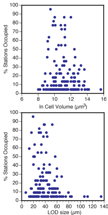
Fig. 7. Scatter plots of occurrence rates of tintinnid species, as a % of stations occupied, among the stations. The top panel shows the lack of relationship of occurrence and lorica volume and the bottom panel shows a similar lack of relation with LOD size. Neither lorica volume nor oral diameter appear linked to average occurrence.
