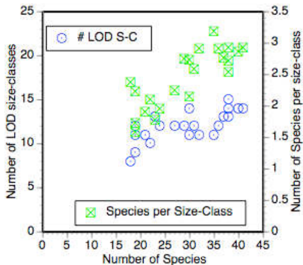
Fig. 6. Species packing in tintinnid communities across the SE Pacific Ocean. Comparing the different stations, both the number of mouth sizes, lorica oral diameter LOD in 4\text{ }\mu\text{m} size-class intervals, and the average number of species per mouth size increased with the number of species.
