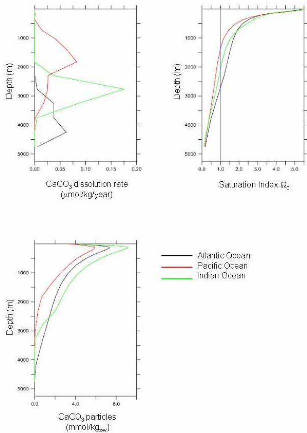
Fig. 3. (a) Average CaCO 3 dissolution rates; (b) Saturation index with respect to calcite; (c) mean concentration of CaCO 3 particles.
