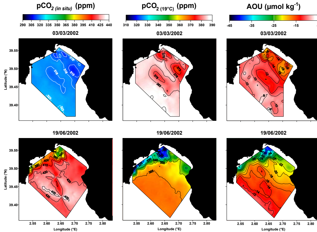
Fig. 8. Surface distributions of pCO 2 ( in situ ) (ppm), pCO 2 normalized to a constant temperature (pCO 2 (19°C), ppm) and AOU (μmol kg -1 ) obtained on 3 March 2002 (EUBAL-I cruise) and 19 June 2002 (EUBAL-II cruise).
