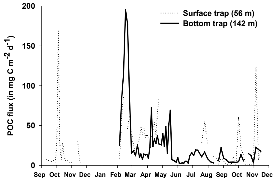
Fig. 5. Particulate Organic Carbon (POC) flux in \text{mg m}^{-2} \text{d}^{-1} in the surface trap (56 m) and the bottom trap (142 m) throughout the year.
