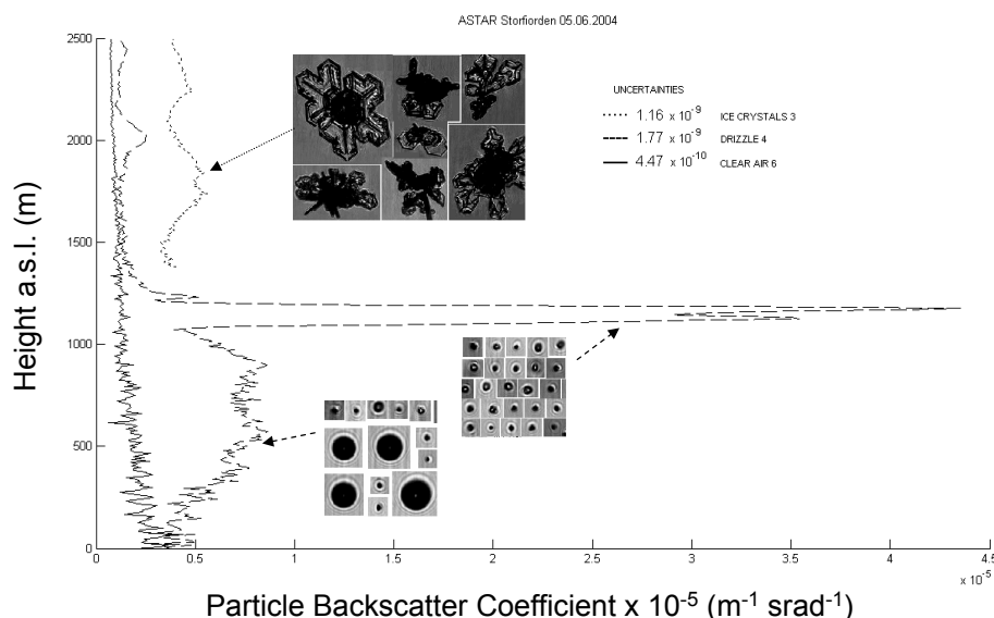
Fig. 5. Vertical profiles of particle backscatter coefficient retrieved for the selected regions in Fig. 3 of: (i) drizzle fallstreak (dashed line), (ii), ice crystals (dotted line) and (iii) cloud-free atmosphere (solid line) from the AMALi measurements at 532 nm. Some CPI images exemplify water drops and ice crystals to related-profiles.
