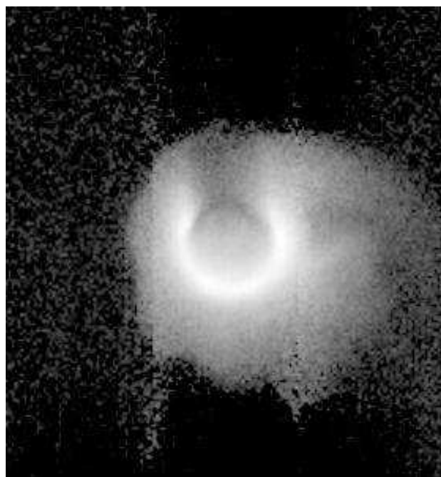
Fig. 6. IMAGE EUV image recorded at 10:32 UT (centre time) on 7 April 2001 when IMAGE was located just past apogee in the Northern Hemisphere.
