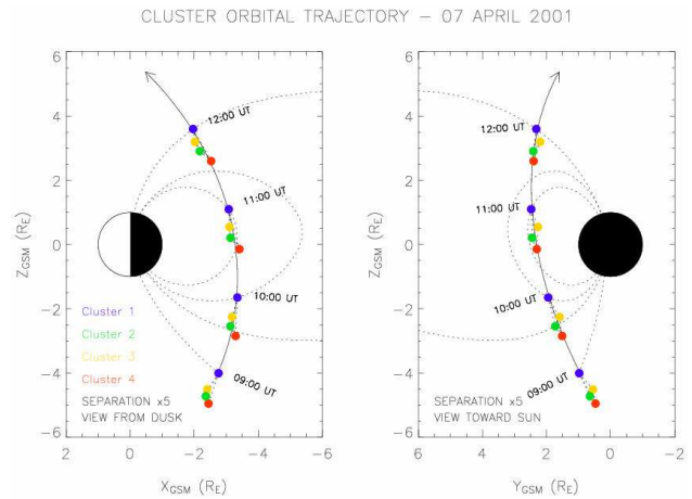
Fig. 2. The trajectory of Cluster 1 satellite in GSM coordinates during 09:00 to 12:00 UT on 7 April 2001. X_{GSM} is positive toward the Sun, Y_{GSM} is positive toward magnetic dusk, and Z_{GSM} is positive toward magnetic north. Cluster 1 locations are highlighted with blue dots at hourly intervals, and the relative locations of the other satellites are exaggerated by a factor of 5.
