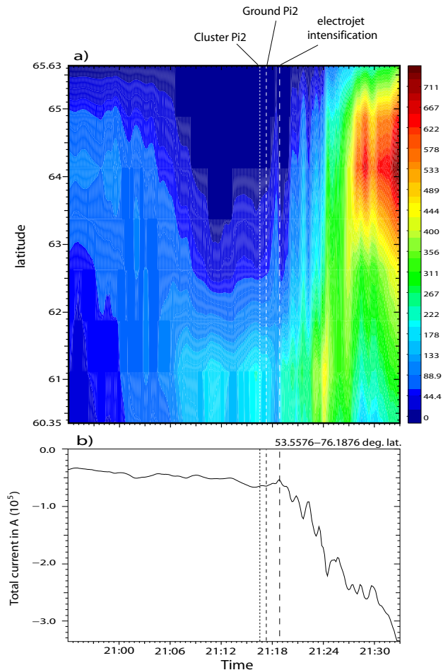
Fig. 6. (a) Latitudinal distribution of the ionospheric westward current (in mA/m) reconstructed from IMAGE magnetometer data (adapted from Sergeev et al., 2005). (b) Total integrated current (in A) of the ionospheric westward current. Dashed lines indicate the onsets of the Cluster Pi2, the ground Pi2, and the intensification of the ionospheric westward current.
