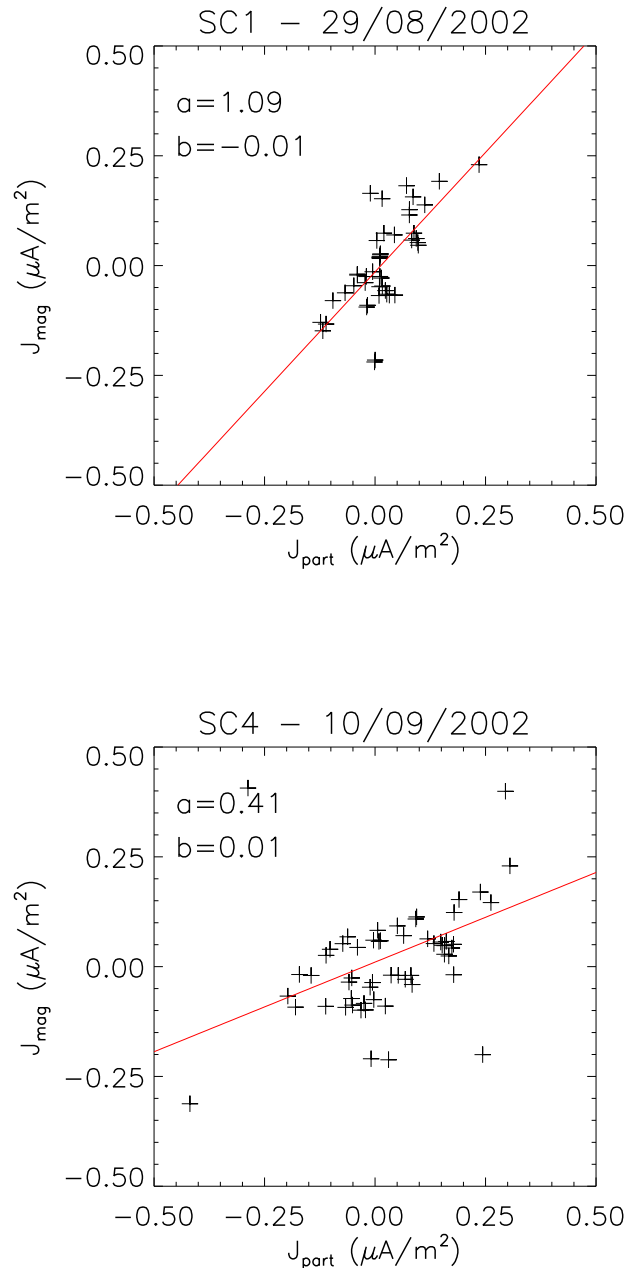
Fig. 5. Least-square linear regression fit (red line) between J_{//part} and J_{//mag} , with a and b : the slope and constant factor of the fit. (Top) for event A (sc-1, 29 August 2002), 16:06–16:15 UT. (Bottom) for event B (sc-4, 10 September 2002), 14:07–14:16 UT.
