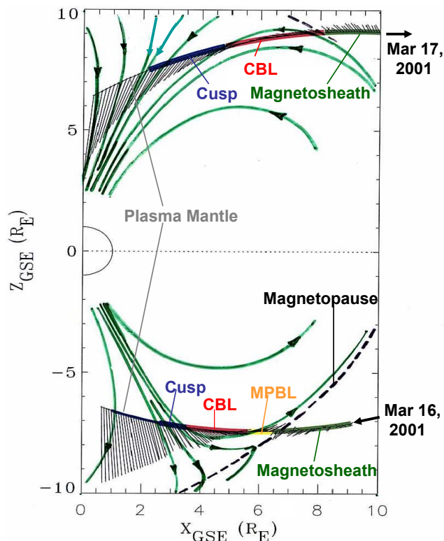
Fig. 1. Trajectories of the Cluster spacecraft for 16 March 2001, 16:00–21:00 UT, and for 17 March 2001, 05:00–10:00 UT, projected onto the x - z plane in GSE coordinates. Measured magnetic field vectors in the x - z plane are overplotted along the trajectories. Also overplotted is a cartoon of magnetic field lines which are consistent with the direction of the measured field vectors on the trajectories. The dashed lines represent the magnetopause. Different colors mark various regions, which include the magnetosheath, closed boundary layer (CBL), the cusp, Magnetopause boundary layer (MPBL), and the plasma mantle.
