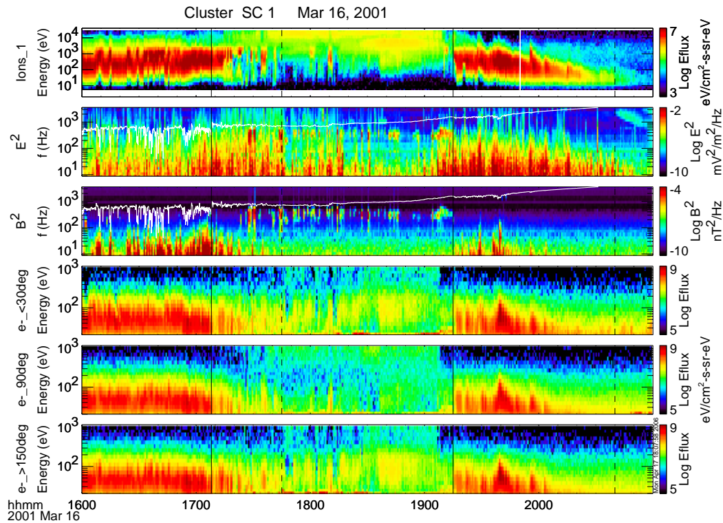
Fig. 5. The same as Fig. 3, but for the period of 16 March 2001, 16:00–21:00 UT.
