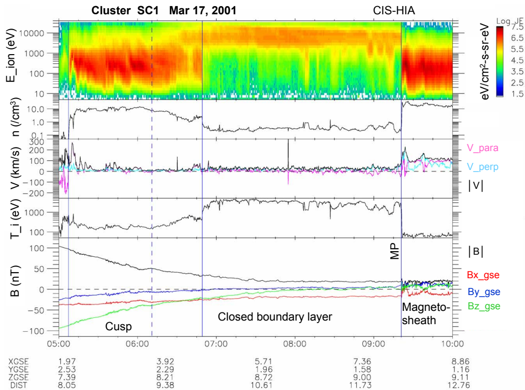
Fig. 2. From top to bottom: The ion energy flux, density, velocity (plotted as components parallel, in red, and perpendicular, in blue, to the ambient magnetic field, and the total velocity in black), temperature, and the magnetic field (in GSE coordinates) variations during the period of 17 March 2001, 05:00–10:00 UT. Vertical lines mark different regions traversed by the spacecraft.
