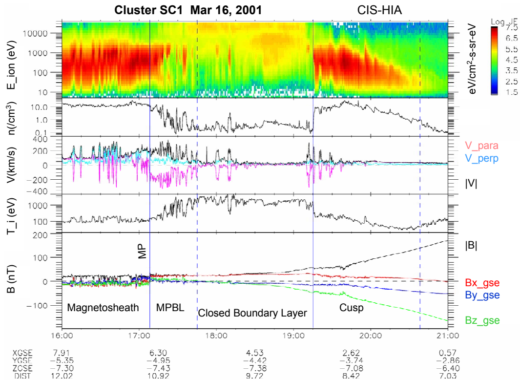
Fig. 4. The same as Fig. 2, but for the period of 16 March 2001, 16:00–21:00 UT.
