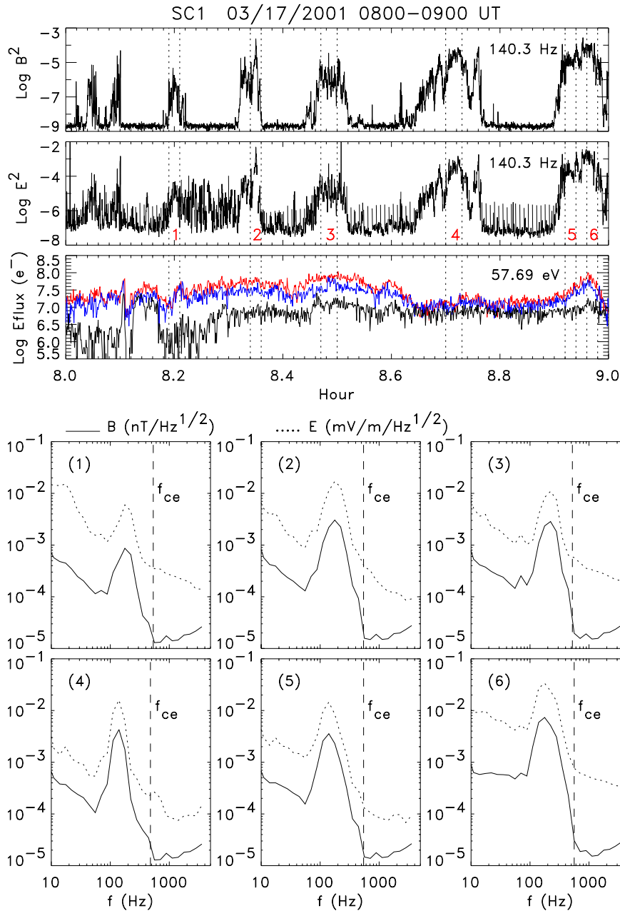
Fig. 6. Panels 1 and 2: The variations of magnetic and electric field wave power density for the period of 17 March 2001, 08:00–0900 UT, detected in a channel with central frequency of 140.3 Hz. Panel 3: The energy fluxes of electrons in the channel of 57.69 eV for three pitch angle ranges: \alpha < 30^\circ (blue), 70^\circ < \alpha < 110^\circ (black), and \alpha > 150^\circ (red), respectively. Six intervals (labeled 1–6 between each pair of vertical dashed lines) are selected for detailed study. The lower part of the figure shows wave amplitude density spectra for the six intervals with the solid curves represent magnetic wave spectra and the dashed curves for the electric wave spectra. The vertical dashed line in each spectra marks the f_{ce} .
