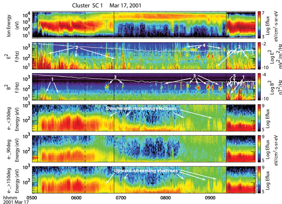
Fig. 3. From top to bottom: (1) The ion energy flux (the same as that in Fig. 2); (2) The sum of the electric field power spectral density (in \text{mV}^2/\text{m}^2/\text{Hz} ); (3) The sum of the magnetic field power spectral density (in \text{nT}^2/\text{Hz} ); (4)–(6) Energy spectra of electrons for pitch angle \alpha < 30^\circ , 70^\circ < \alpha < 110^\circ , and \alpha > 150^\circ , respectively. The vertical black lines marked the boundaries between different regions as in Fig. 1. Numbers in panels 2 and 3 mark wave mode observed: “1” for the broadband magnetic noise; “2” for the broadband electrostatic emissions; “3” for the CBL whistler mode waves; “4” for the narrow-band electrostatic whistler waves; and “5” for the lion roars.
