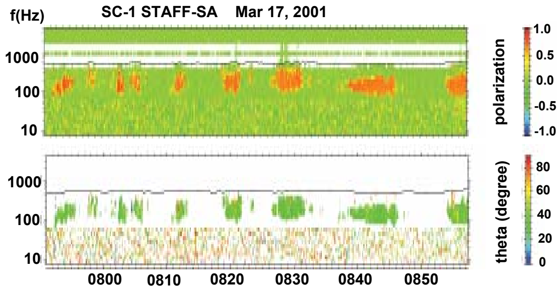
Fig. 7. Results from computer program PRASSADCO showing the polarization (upper panel) and the wave angle (lower panel) of the waves for the interval on 17 March 2001, 07:51–08:57 UT.
