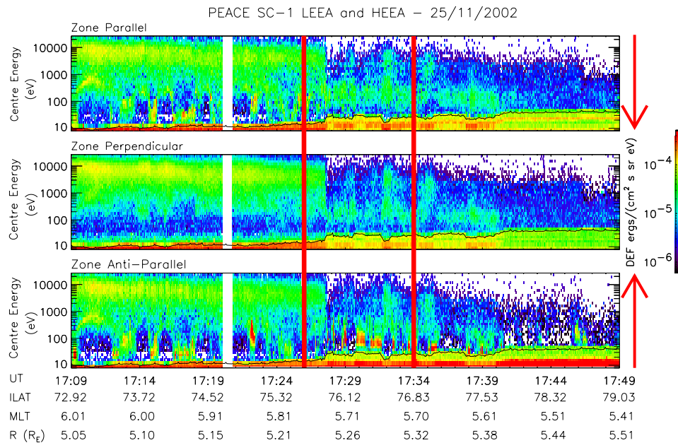
Fig. 6. Overview of PEACE data for the bipolar electric field event in Fig. 4. The panels are the same as in Fig. 2. However this event occurs in Northern Hemisphere, so down-going electrons are found in the first panel and up-going electrons are found in the third panel, as indicated with arrows. The vertical red lines mark the shorter interval displayed in Fig. 5.
