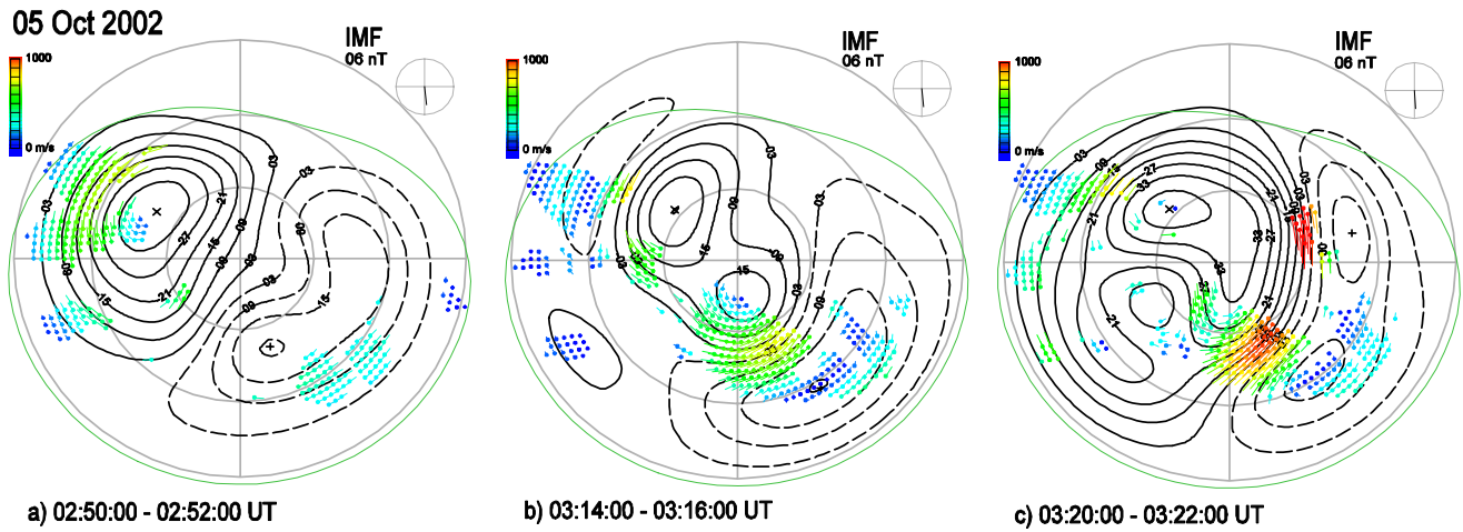
Fig. 3. SuperDARN map potential plots for 5 October 2002 in the Northern Hemisphere polar cap within 60 deg (geographic coordinates) with IMF value and direction indicated. Noon local time is at the top of the plot. (a) 02:50 to 02:52 UT; (b) 03:14 to 03:16 UT; (c) 03:20 to 03:22 UT.
