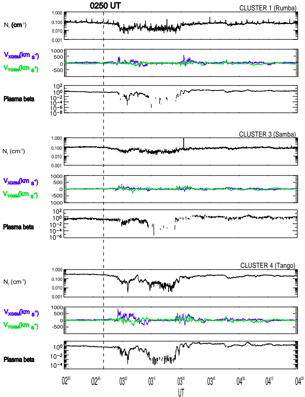
Fig. 8. Cluster CIS ion data from spacecraft 1, 3 and 4 for 5 October 2002, from 02:30 to 04:30 UT; density, x and y velocity components (GSM coordinates) and plasma beta are shown for each spacecraft.
