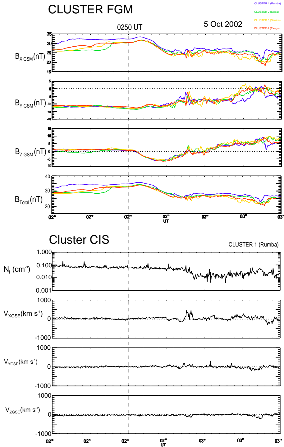
Fig. 11. (b) zoomed view for the 02:40 to 03:10 UT interval: B_x , B_y , B_z and B_{\text{total}} Cluster FGM data from the four spacecraft and density, V_x , V_y and V_z CIS data from Cluster 1.
