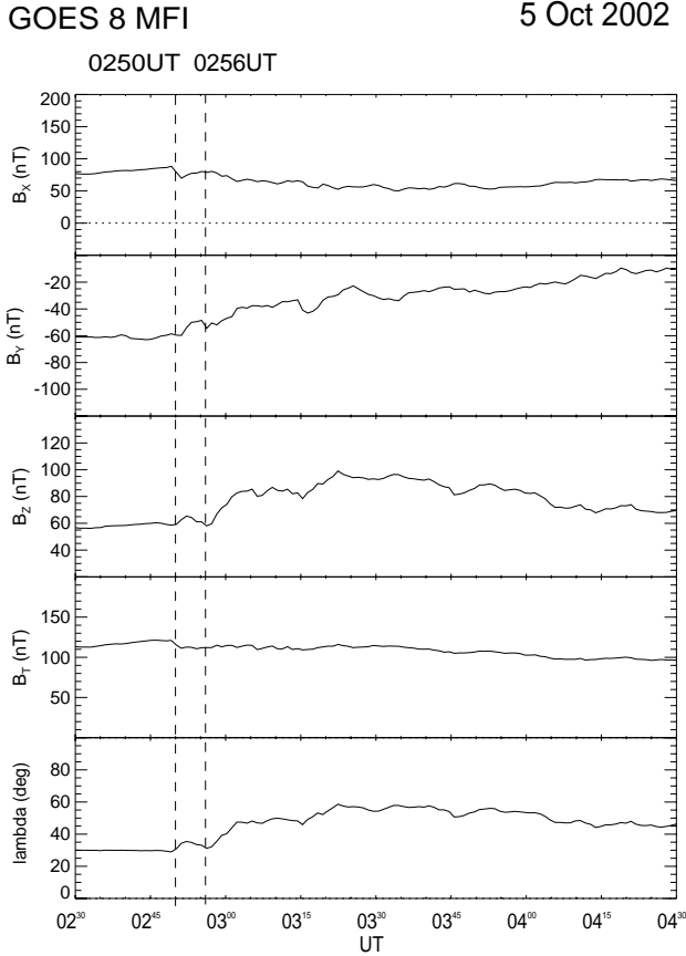
Fig. 5. GOES 8 magnetometer data for 5 October 2002, from 02:30 to 04:30 UT. B_x , B_y , B_z components of magnetic field, total magnetic field, and lambda, where \tan \lambda = B_z / \sqrt{(B_x^2 + B_y^2)} , are shown.
