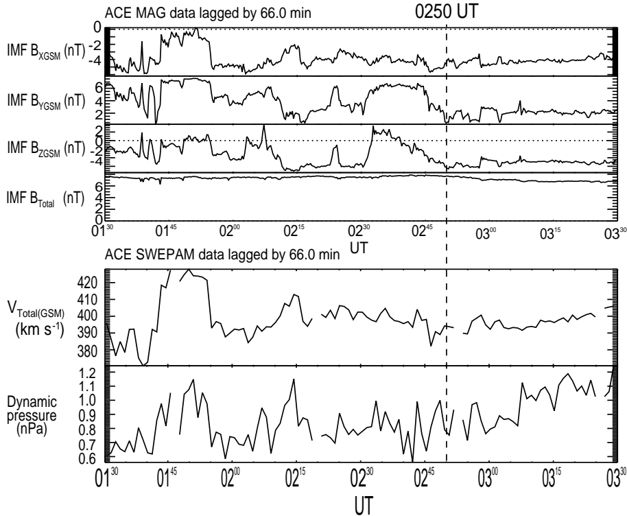
Fig. 4. ACE MAG and SWEPAM data for 5 October 2002, from 01:30 to 03:30 UT, lagged by 66 min. Top panel depicts MAG data: B_x , B_y , B_z components of magnetic field and the total magnetic field, in GSM coordinates. Bottom panel depicts SWEPAM data: total velocity and dynamic pressure.
