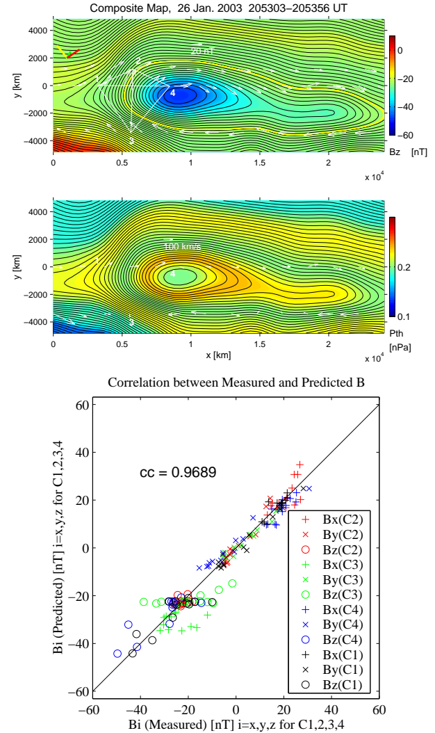
Fig. 7. Field and pressure maps and associated scatter plot for FTE 4.
