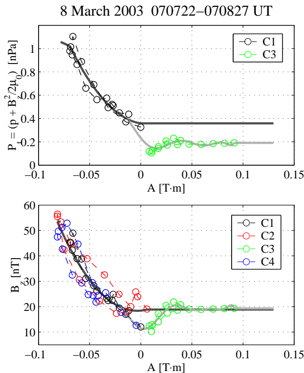
Fig. 2. Transverse pressure P_t = (p + B_z^2 / (2\mu_0)) (top) and axial magnetic field component B_z (bottom) versus partial magnetic vector potential A for FTE 2. The fitted curves are polynomial functions of A ; P_t(A) is determined using the data points from C1 and C3 for which the CIS/HIA and FGM instruments were both operative, while B_z(A) is determined using those from all four spacecraft. The black branch of the curves is used for reconstructing the magnetic flux rope and magnetosheath region (seen in the upper part of the maps in Fig. 3), while the gray branch is for the magnetospheric region (lower part).
