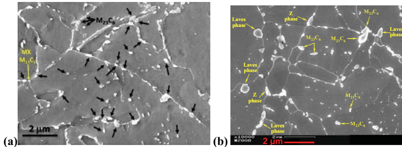
Figure 9 : Microstructure of ASME Grade 91 steel after creep (FEG-SEM, SE mode): (a) at 500°C for 4317h (arrowed precipitates are all probably M_{23}C_6 ); (b) at 600°C for 113431h
