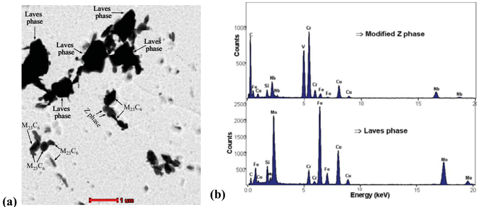
Figure 8 : (a) Precipitates in Grade 91 steel after creep at 600°C for 113431h (TEM, bright field, extractive replica)
