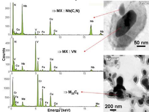
Figure 2: Identification of precipitates from replicas of Grade 91 base metal (EDX, STEM)
