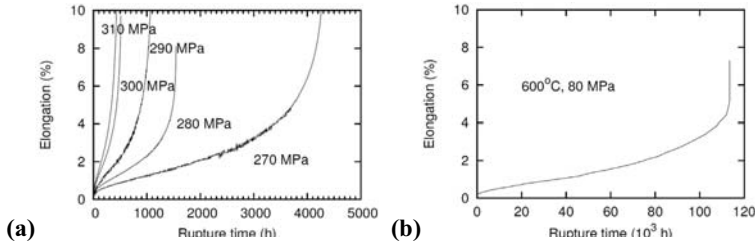
Figure 3: (a) Creep curves at 500°C, (b) Creep curve at 600°C
