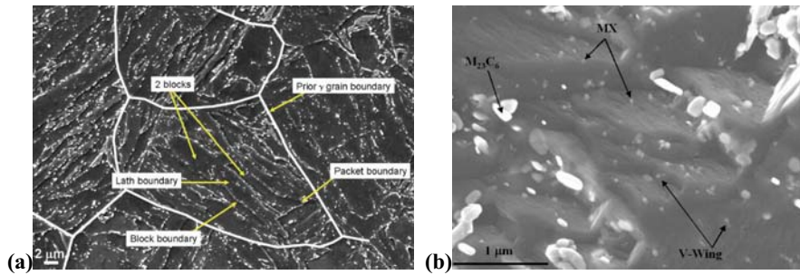
Figure 1: Typical microstructure and precipitates of as-received Grade 91 base metal (SEM) (a) Vilella etched bulk, some austenite grain boundaries are underlined in white (b) Extractive carbon replica showing various kinds of precipitates
