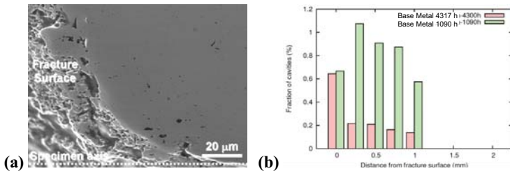
Figure 6: (a) Creep damage after short term creep exposure (4317h) at 500°C (SEM, SE); (b) Evolution of the area fraction of cavities along the specimen axis at 500°C
