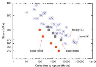
Figure 11 : Creep data at 500°C for base metal and welded joint [9, 10] Solid symbols are for results of the present study
