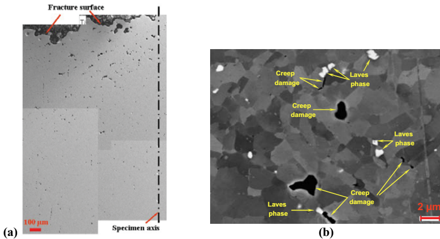
Figure 7: Creep damage and microstructure after long term creep (11343h) at 600°C (a) Secondary electrons mode, SE; (b) Backscattered electrons mode, BSE
