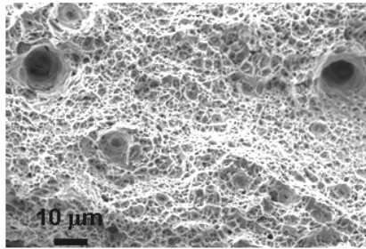
Figure 4: Fracture surfaces of crept base metal specimen after 4317h at 500°C (SEM)
