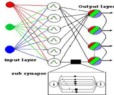
Fig. 2. Network architecture
