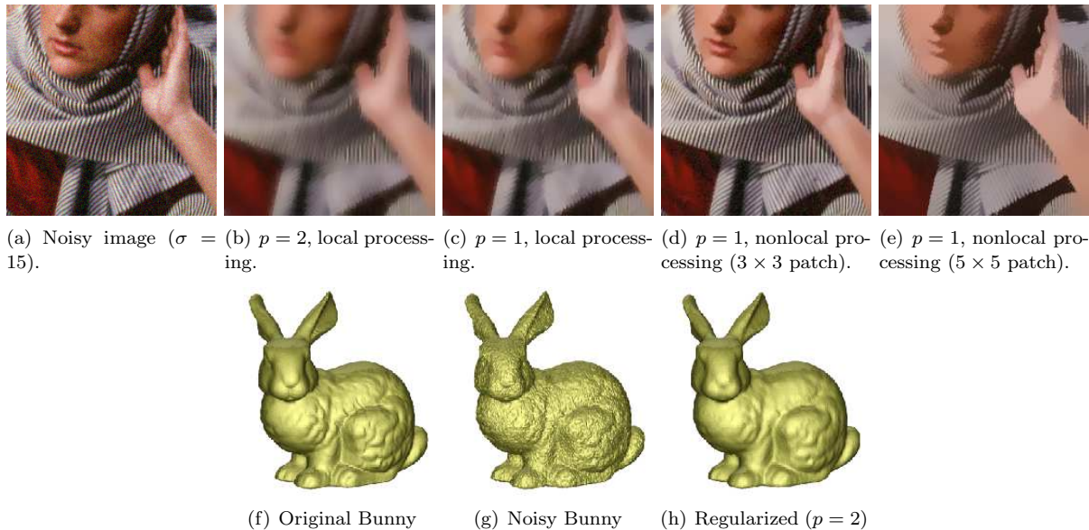
Figure 1. Processing examples for different values of p for local and nonlocal image and mesh processing.
