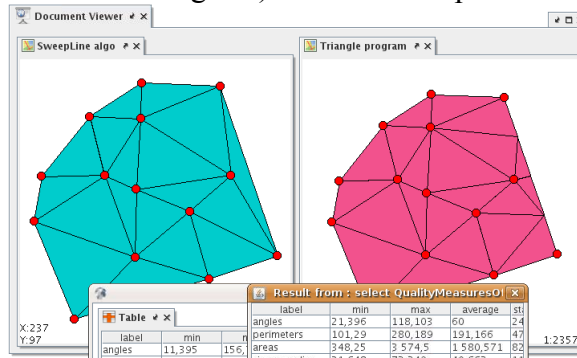
Figure 1. The influence of the Delaunay refinement algorithm on the triangulation. Shewchuk's implementation (on the right side) introduces some Steiner points to obtain a greater minimum angle.
