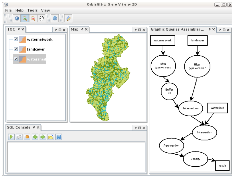
Figure 8: Use case translation in the graphic query builder context
