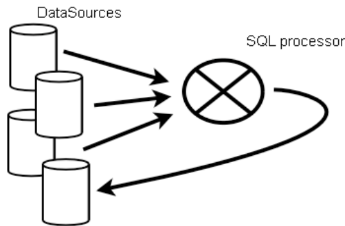
Figure 3: Data sources feedback after processing: implementation of materialized views
