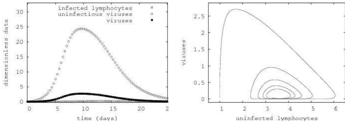
Figure 8. Numerical results for our model. Case where a seropositive state is stable ( \tau = 10, \zeta = 1 ). Relatively short time evolution on the left (25 days) and phase plane for lymphocytes and viruses on the right for a 600 days evolution.
