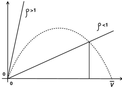
Figure 6. Two characteristic shapes of the curves V \mapsto \rho V and V \mapsto J(V(\bar{V} - V)/\bar{V}) (dotted) for \eta > 0 .
