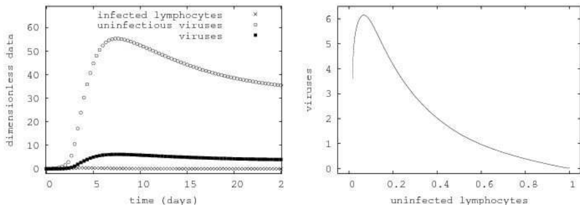
Figure 10. Numerical results for our model. Case where a seropositive state is stable ( \tau = 1, \zeta = 10 ). Relatively short time evolution on the left (25 days) and phase plane for lymphocytes and viruses on the right for a 600 days evolution. The effect of the infection is to reduce drastically the efficacy of the immune system.
