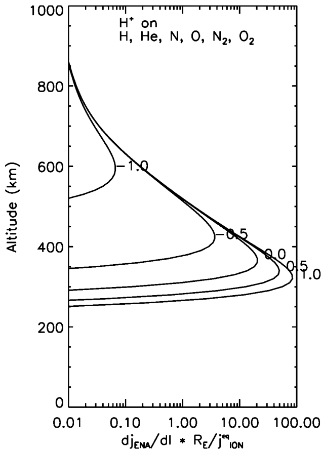
Fig. 16. The ENA production function \partial j_{\text{ENA}}/\partial l \cdot R_E/j_{\text{ION}}^{\text{eq}} (see the text) for 40 keV \text{H}^+ ions plotted as a function of altitude for various values of the pitch angle, assuming a six-component exosphere ( \text{H} , \text{He} , \text{N} , \text{O} , \text{N}_2 and \text{O}_2 ).
