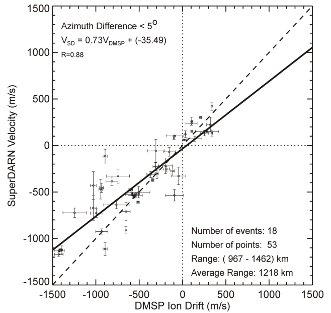
Fig. 5. A scatter plot of the Stokkseyri l-o-s velocity versus the DMSP cross-track ion drift for 18 joint events at radar ranges of \sim 1000 – 1500 km.
