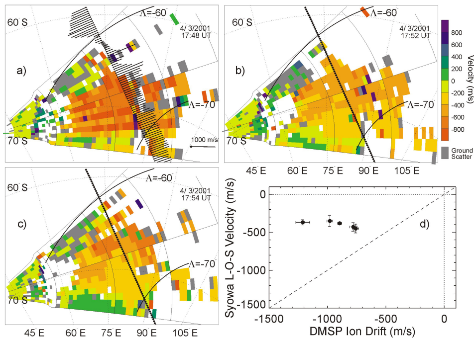
Fig. 7. (a)–(c) Syowa-East l-o-s velocity maps for 17:48, 17:52 and 17:54 UT and the DMSP cross-track ion drift observed between \sim 17:49 and 17:53 UT for the event of 4 March 2001. Panel (d) is a scatter plot of the radar velocity versus DMSP ion drift for the points in panel (b) with the difference between the radar and satellite directions of less than 5^\circ and the difference in time of less than 2 min.
