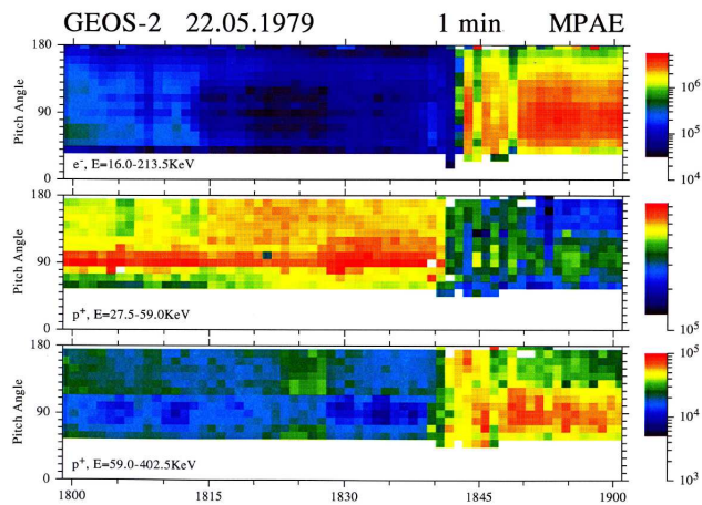
Fig. 7. Pitch angle flux intensities for high energy electrons and ions recorded on GEOS-2.
