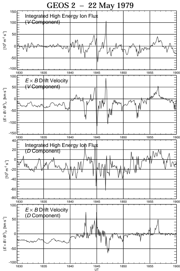
Fig. 8. GEOS-2 measurements as functions of time. From top to bottom: 1. High energy ( >33 keV) radial ion flux intensity; 2. Calculated radial \mathbf{E} \times \mathbf{B} -drift velocity; 3. High energy ( >33 keV) azimuthal ion flux intensity; 4. Calculated azimuthal \mathbf{E} \times \mathbf{B} -drift velocity.
