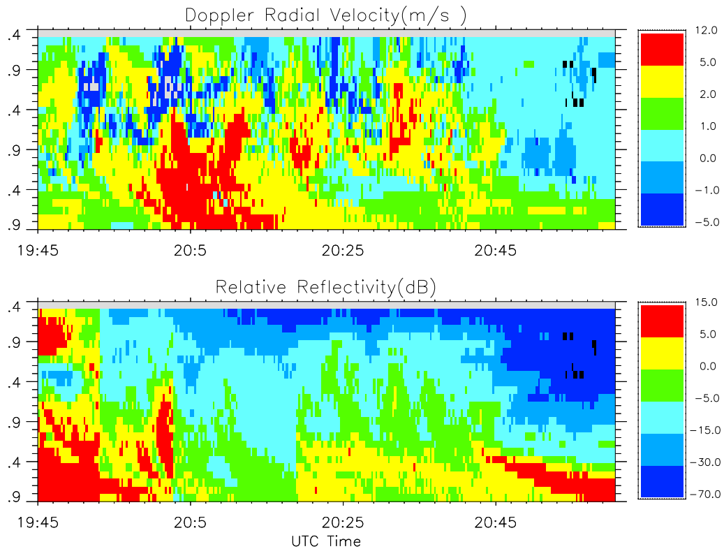
Fig. 3. UHF Strato-tropospheric radar: the lower plot represents the relative reflectivity in color scale (relative dB) as a function of altitude and time; the upper plot represents the Doppler velocity in the vertical beam in color scale (m/s) as a function of altitude and time; positive values correspond to upward motion.
