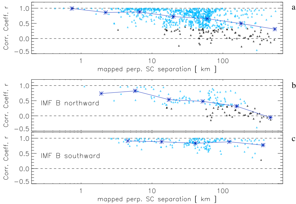
Fig. 9. (a) Correlation coefficients of 1-h intervals of 60-s smoothed \tilde{V}_s vs. mapped spacecraft separation distances transverse to the magnetic field; correlation coefficients above the significance threshold are colored blue, the others black; (b) and (c) same as (a), except the subset of cases with steady IMF have been separated into IMF northward and southward, respectively. The asterisks interconnected by straight lines show the average trend.
