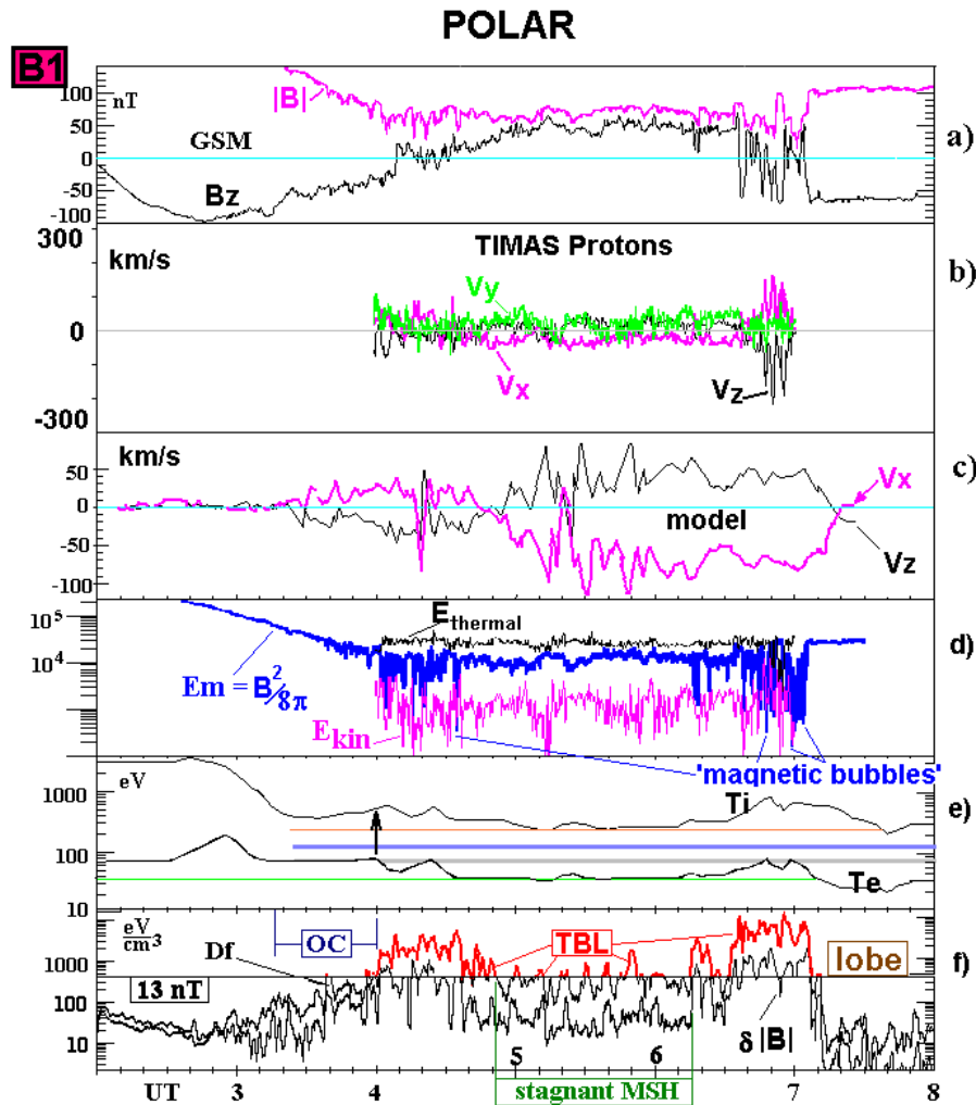
Plate B1. Particle and field parameters on Polar on 29 May 1996. Panel (a): the magnetic field |B| (violet) and GSM B_z (black). Panel (b): vector velocities of protons by the TIMAS spectrometer, V_x , V_y and V_z are marked by violet, green and black colors, respectively. Panel (c): GSM V_x (violet) and V_z (black) components of ion velocity from the global MHD model (Fedder et al., 1995). Panel (d): the kinetic ion energy density (violet), the ion thermal energy density (black), and the magnetic energy density (blue); the ion densities are shown only at 04:00–07:00 UT. Panel (e): the average ion energy T_i (upper black line) from HYDRA, the minimum T_i from Polar in the MSH (brown), the characteristic T_i in the MSH from Interball-1 (thick blue line) at 04:00 UT (marked by the vertical arrow), T_i in the MSH from the MHD model at 04:00 UT (gray line), average electron energy T_e (the lower black line) from HYDRA, and minimum T_e in the MSH / TBL (green). Panel (f): the magnetic field variations calculated in the same way as on panel (f) of Plate A2; the TBL is red-colored in Df , upper curve, the characteristic regions marked according to Plate A1.
