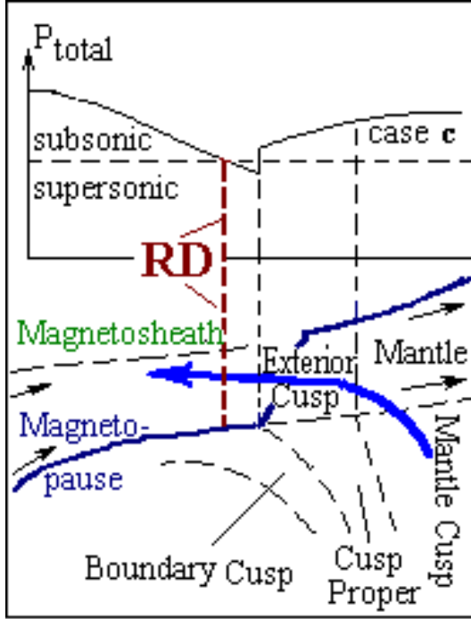
Fig. 1. Yamauchi and Lundin (1997) “Laval nozzle” model sketch; thick arrow infers Interball-1 orbit (see Plate A2). See text for further details.
