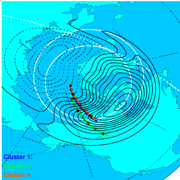
Fig. 2. Magnetic footpoints of the Cluster satellites (SC1 blue, SC3 green, SC4 red) during their cusp crossing at 25 July 2001, to illustrate their spatial separation. Also shown are convection cells derived from SuperDARN radar observations for the time period from 23:00 UT to 23:30 UT.
