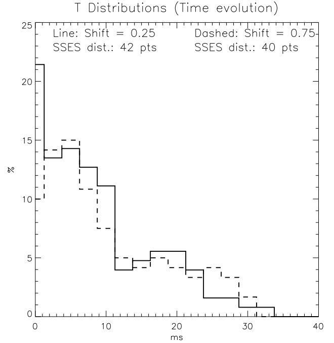
Fig. 7. Correlation time in the first (bold line) and second (dashed line) halves of the event.
