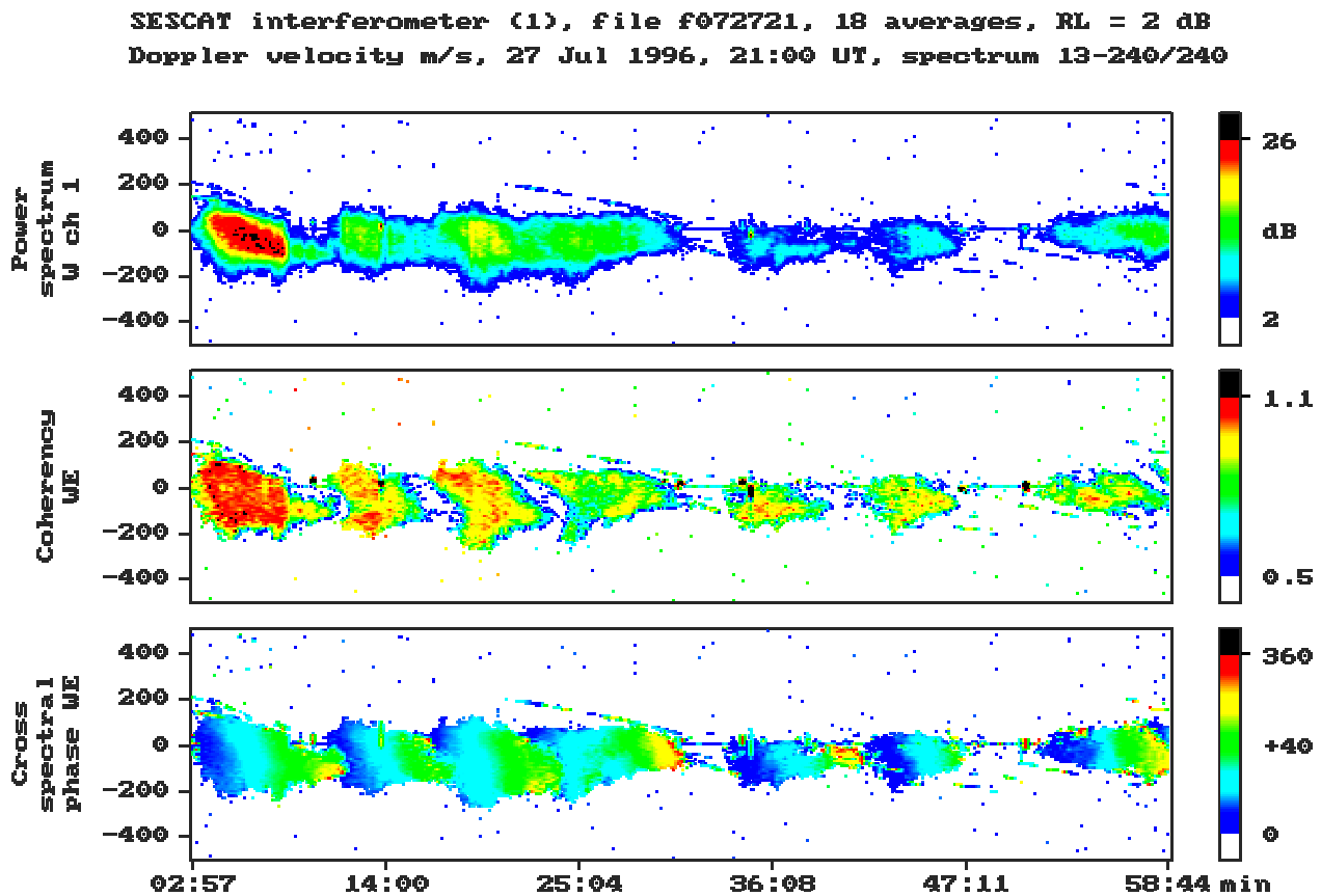
Fig. 7. Power spectra and cross-spectral Doppler spectrograms for a typical example of quasi-periodic (QP) echoes having, on average, a period of \sim 8 min. As seen, the QP echoes are basically a sequence of individual plasma structures which are unstable as they move across the radar beam.
