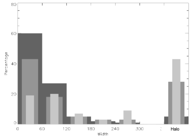
Fig. 8. In light grey: width (in ^{\circ} ) distribution for the CMEs identified in column 7 of Table 1. In dark grey: same histogram for the CMEs identified in column 6 of Table 1. In black: same histogram for all the CMEs identified in LASCO during the same period.
