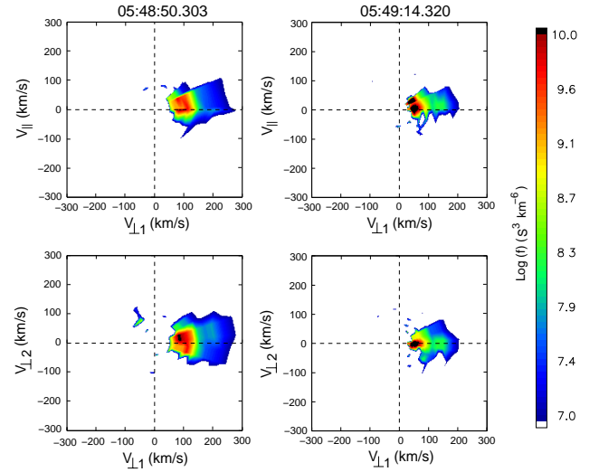
Fig. 5. Top: ion distribution function in a plane ( V_{\parallel} , V_{\perp 1} ). Bottom: in a ( V_{\perp 1} , V_{\perp 2} ) plane. The distributions are averaged on board over 12 s. The ( V_{\parallel} , V_{\perp} ) plane contains the onboard computed bulk velocity. Left, distribution starting at 05:48:50.303. Right, starting at 05:49:14.320 (see text and Fig. 3). These data come from the CIS-2 sensor (no mass resolution).
