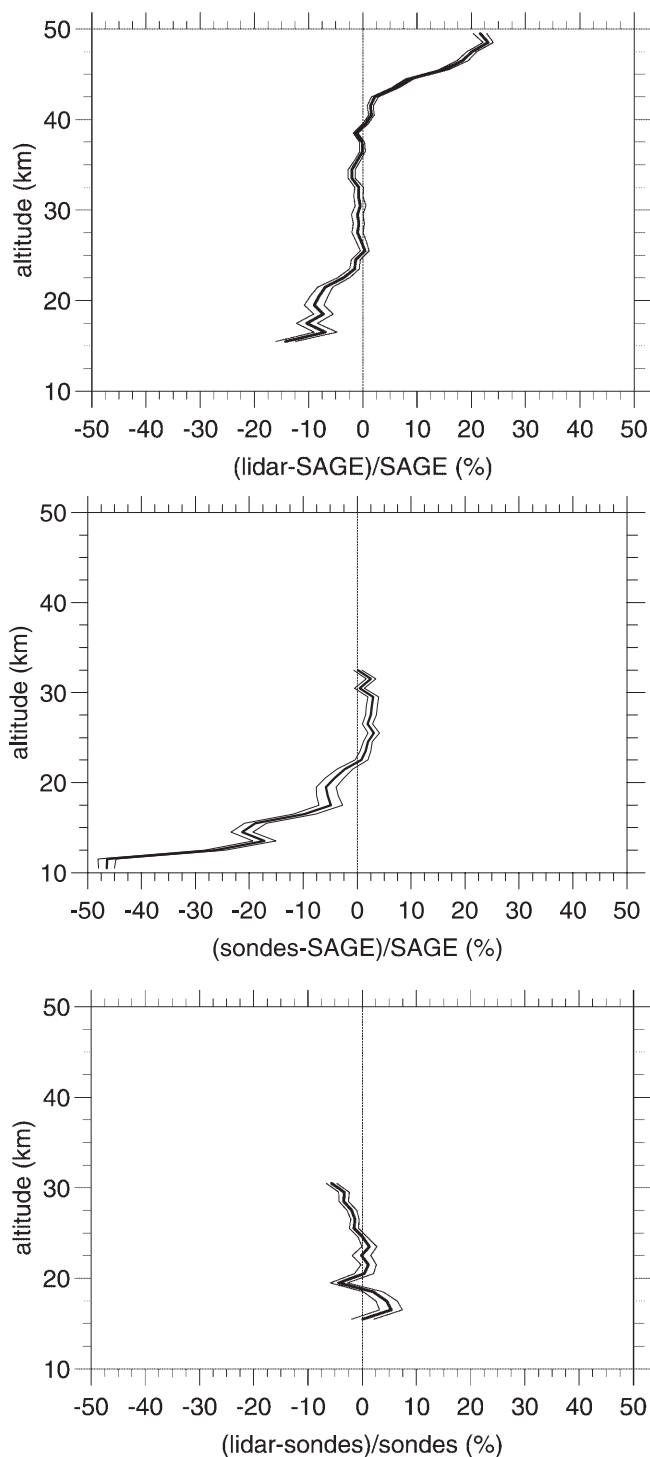
Fig. 5. Same as Fig. 4, with data sets being restricted to only measurements in temporal coincidence
