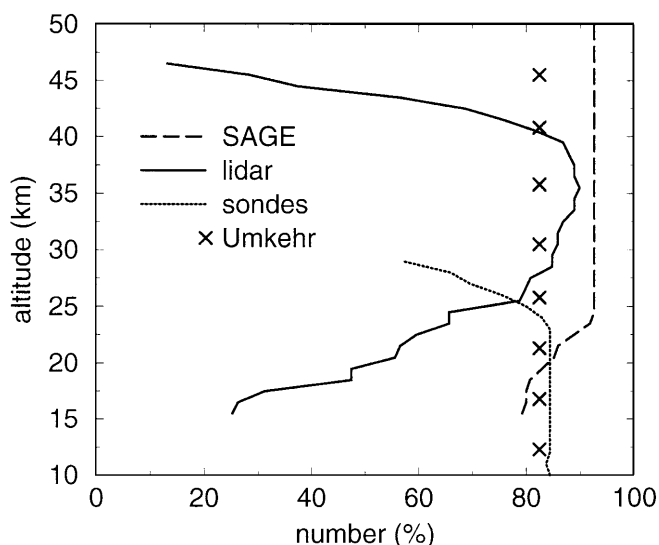
Fig. 2. Altitude dependence of the percentage ratio between the number of monthly means available for each instrument and the total number of months over the whole period considered in this study (see Table 1)
