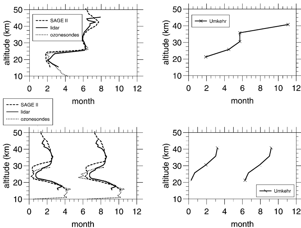
Fig. 7. Altitude dependence of the phases of the annual ( top row ) and semi-annual ( bottom row ) variations as derived from SAGE II, lidar, ozonesonde ( left column ) and Umkehr measurements ( right column ) at OHP. The phase of the semi-annual variation is given with a 6 months period. For Umkehr measurements, the altitude of reference is the centre altitude of the Umkehr layer
