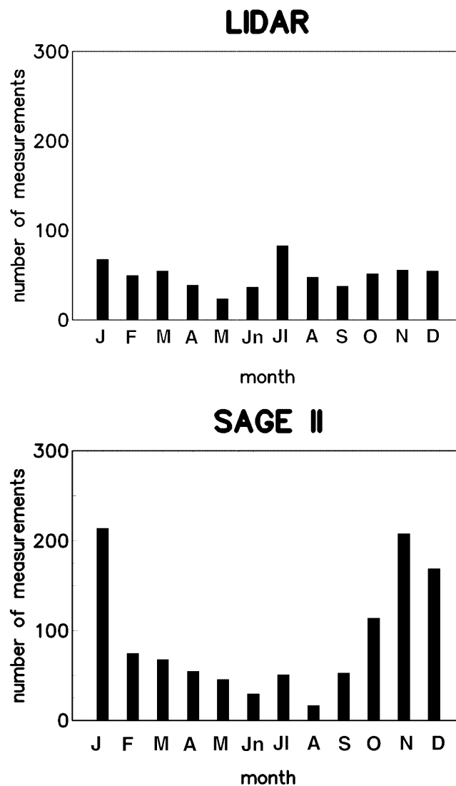
Fig. 1. Total number of measurements per month for lidar measurements between 1986 and 1995 ( upper panel ) and for SAGE II measurements between 1984 and 1995 ( lower panel ) at OHP
