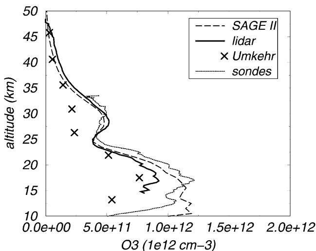
Fig. 3. Mean vertical ozone profiles ( top ) and corresponding standard deviation ( 1\sigma ) ( bottom ) between 10 km and 50 km for SAGE II, lidar, ozonsondes and Umkehr measurements at OHP
