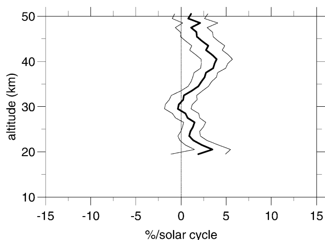
Fig. 10. Solar contribution with 1\sigma standard deviation limits as a function of altitude as derived from SAGE II measurements at OHP. Values are given in % per solar cycle
