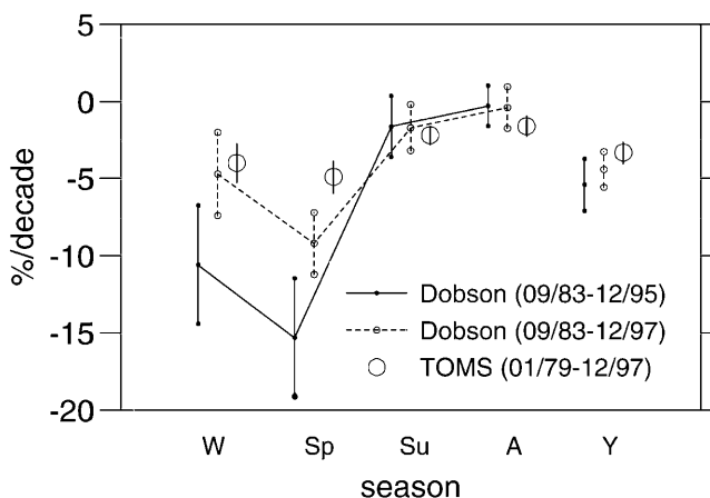
Fig. 8. Ozone trends derived from Dobson measurements at OHP between September 1983 and December 1995 and between September 1983 and December 1997 (WMO, 1998); ozone trends derived from TOMS measurements between January 1979 and December 1997 (WMO, 1998). Trends are given in % per decade with a 1\sigma uncertainty limit for the four seasons winter, spring, summer, autumn ( W , Sp , Su , A ) and for the whole year ( Y ). The seasonal variations, the QBO and the 11-year solar cycle have been removed
