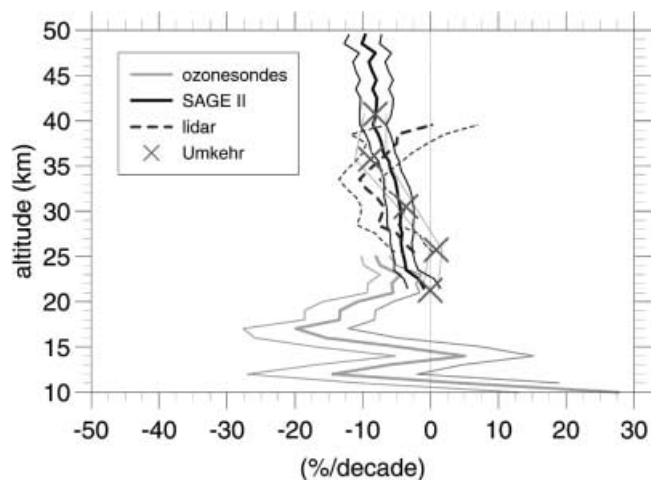
Fig. 9. Ozone trends as a function of altitude derived from SAGE II, lidar, ozonesondes, and Umkehr measurements at OHP. Trends are given in % per decade with 1\sigma uncertainty limits after removal of the seasonal variations, the QBO and the 11-year solar cycle
