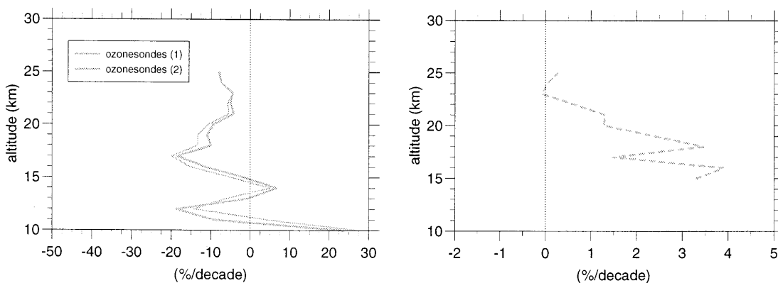
Fig. 11. Ozone trends in %/decade as a function of altitude as derived from ozonesonde measurements at OHP ( left panel ); curve (1) is the same as in Fig. 9, i.e. without considering the aerosol effect;
