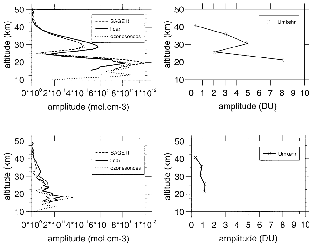
Fig. 6. Altitude dependence of the amplitudes of the annual ( top row ) and semi-annual ( bottom row ) ozone variations as derived from SAGE II, lidar, ozonesonde ( left column ) and Umkehr measurements ( right column ). For Umkehr measurements, the altitude of reference is the centre altitude of the Umkehr layer
