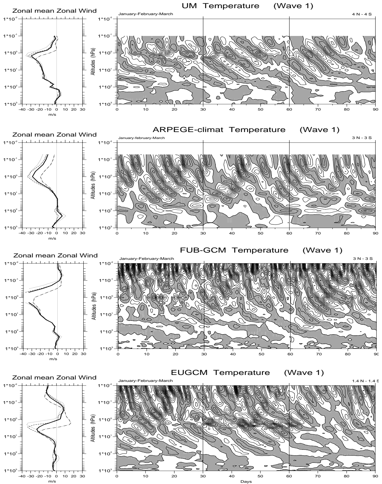
Fig. 6. Time-height section of temperature zonal wave 1 averaged over an equatorial band at 0^{\circ} longitude for the time period Jan-Mar and Apr-Jun for the UM, ARPEGE-climat, FUB-GCM and EUGCM models. Positive values are shaded and the contour interval is 1 K. The solid lines of the left panel show the zonal wind profiles averaged over the 3 months Jan-Feb-Mar and Apr-May-Jun; dotted lines correspond to January and April, dashed lines to February and May and dash-dotted lines to March and June.
