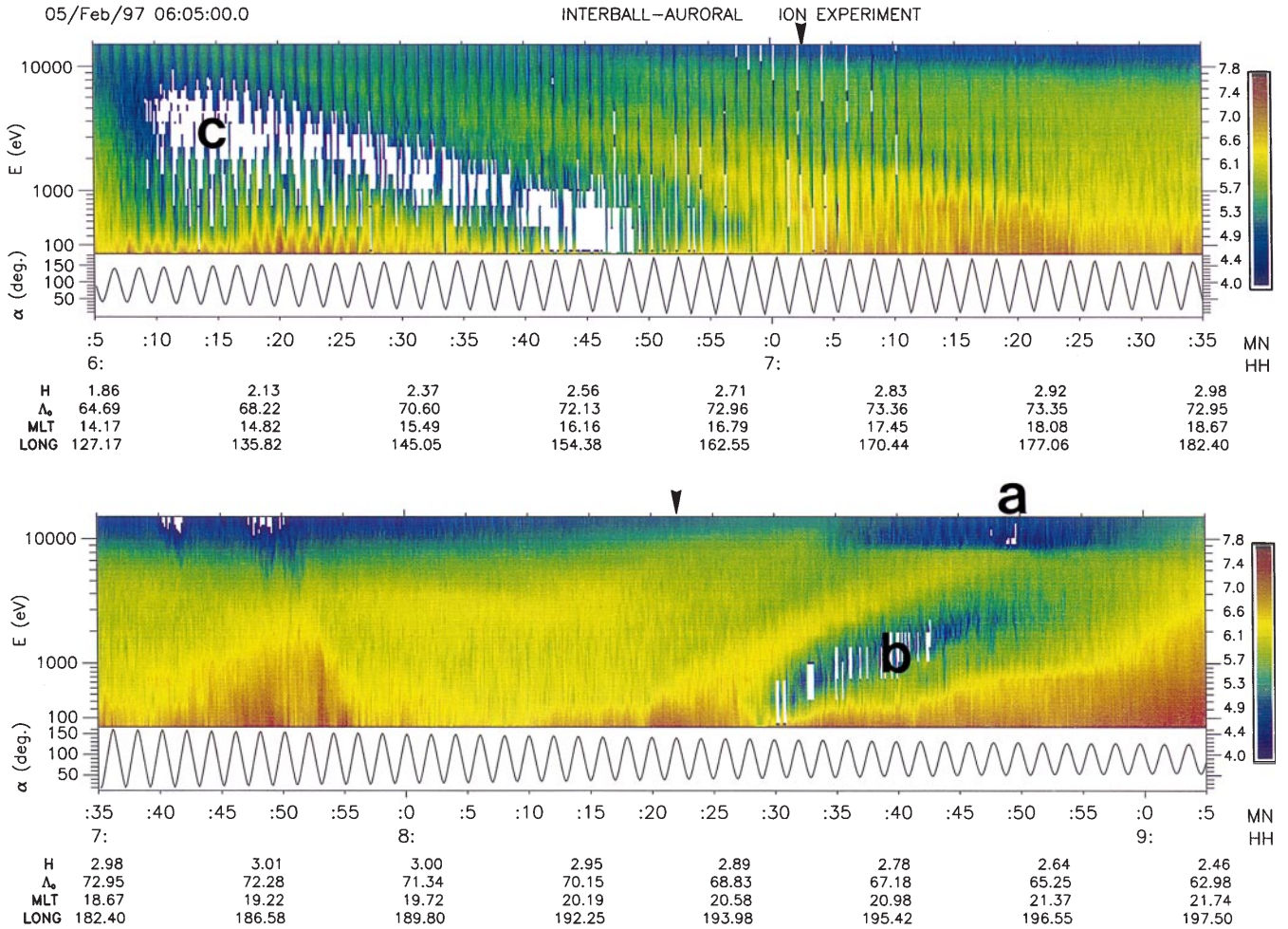
Fig. 2a, b. Ion energy-time spectrograms recorded by INTERBALL-Auroral on February 5, 1997: a in the afternoon sector (from 0605 UT until 0735 UT), b in the evening sector (from 0735 UT until 0900 UT).
