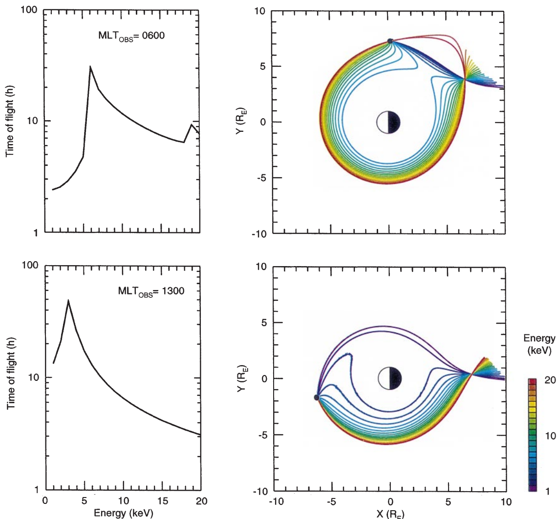
Fig. 5. Model H^+ trajectories in the Tsyganeko (1998) model: (right) equatorial crossing points, (left) time of flight versus initial energy. The test protons are traced backward in time from an observation
