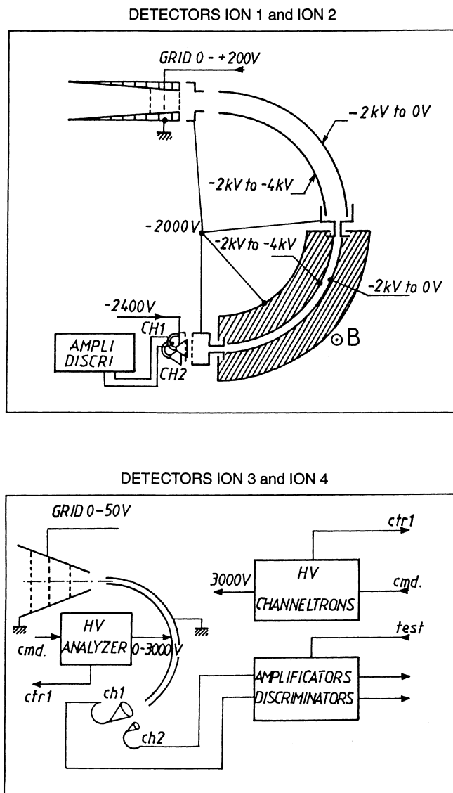
Fig. 1. Block diagram of the ion mass spectrometers (top) and the electron sensors (bottom)
