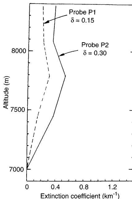
Fig. 8. Vertical profiles of the extinction coefficient at 1.06\ \mu\text{m} deduced from measurements of two PMS 2D-C probes (P1, P2) during the sampling at different levels of a cirrus cloud
