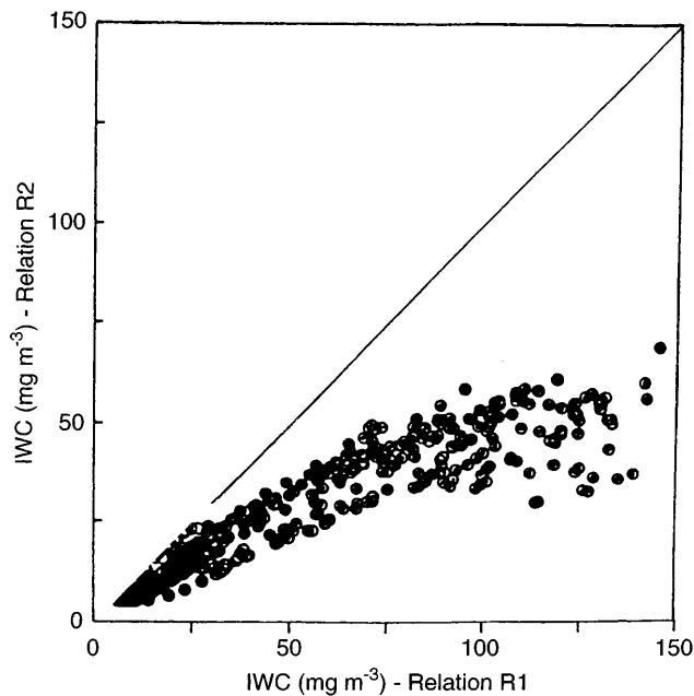
Fig. 9. Comparison of the IWC obtained by using two size-mass relationships ( R1 : bullet-rose; R2 : irregular) applied to the same data set (cirrus measurements performed near -30^{\circ}\text{C} during the mission 210 of the International Cirrus Experiment ICE/EUCREX)
