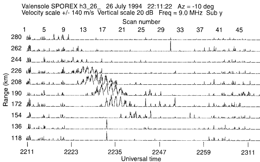
Fig. 4. Time evolution of E-region aspect sensitive echoes at 9 MHz in azimuth 10^{\circ}\text{W} , in the time-period 2211–2314 UT. The Doppler spectrum at any cell is logarithmic on a 20-dB scale with the Doppler velocity ranging from -140 to 140 m/s. A scattering region forming a band with a negative range rate of about 90–110 m/s is observed between 2223 and 2241 UT
