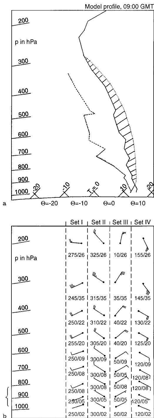
Fig. 3. a Initialisation profile of dew point and dry bulb temperatures for the numerical simulations. The shaded area represents the convectively available potential energy (CAPE) of the air masses. b Profiles of wind vectors given in degrees and knots
