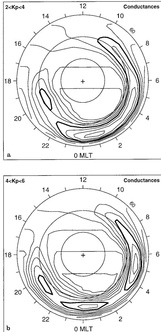
Fig. 1a,b. Isocontours of Hall conductances represented in polar maps between the north pole and 60^\circ invariant latitude, with the MLT indicated on the external circle. The contour interval is 2 mhos and the bold line corresponds a to 10 mhos for 2 < Kp < 4 and b to 13 mhos for 4 < Kp < 6
