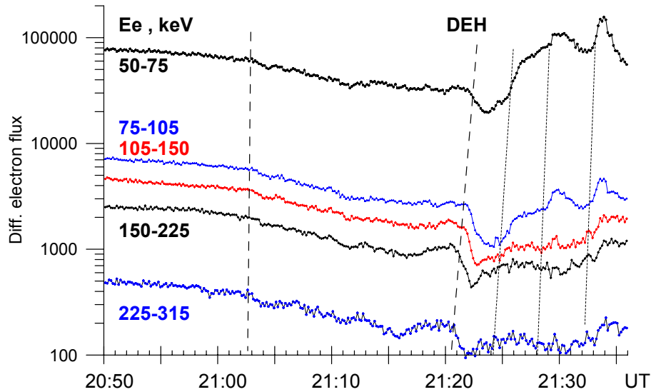
Fig. 6. Differential fluxes of energetic electrons recorded at the LANL 02A spacecraft ( \sim 02:00 LT). The only feature around substorm onset at GEO orbit was the drifting electron hole corresponding to the injection of depressed particle flux at around 21:20 UT.
