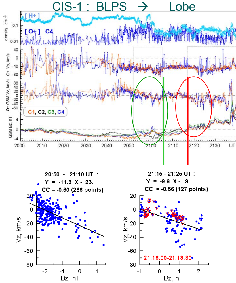
Fig. 9. Top: H^+ and O^+ plasma densities, O^+ perpendicular flows at C1 and C4 spacecraft and B_z -variations at four Cluster spacecraft. Bottom: V_z – B_z correlation plots for time periods, including the pseudo-breakup and the substorm onset.
