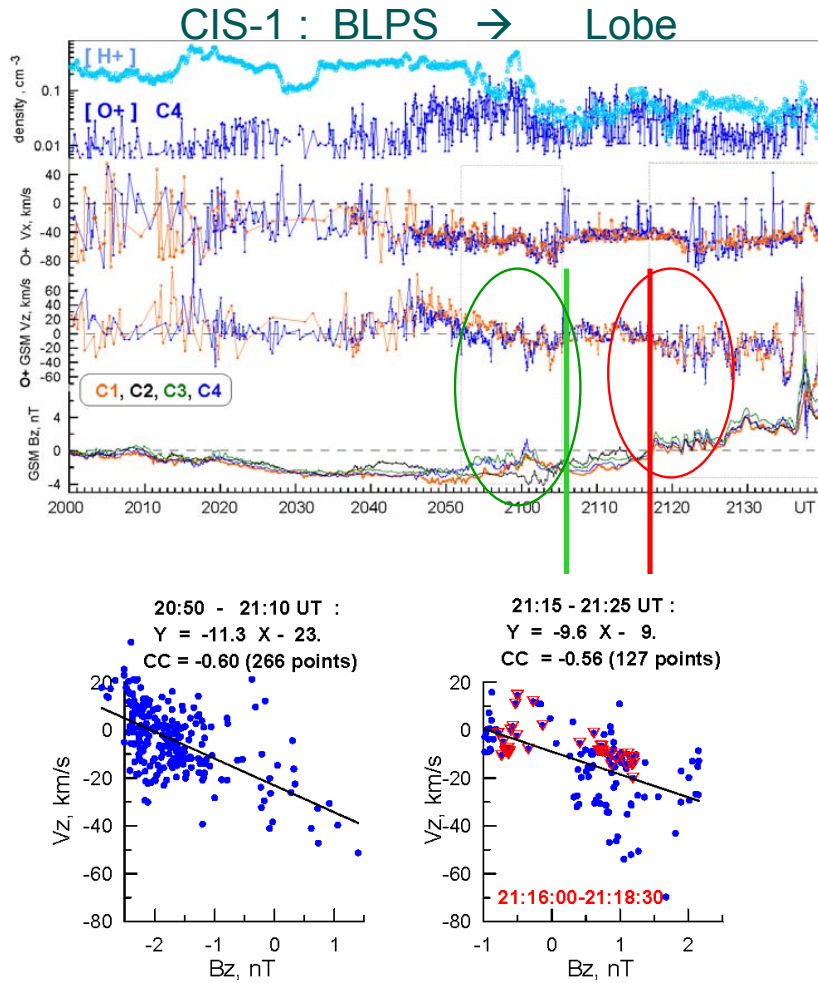
Fig. 9. Top: H^+ and O^+ plasma densities, O^+ perpendicular flows at C1 and C4 spacecraft and B_Z -variations at four Cluster spacecraft. Bottom: V_Z-B_Z correlation plots for time periods, including the pseudo-breakup and the substorm onset.
