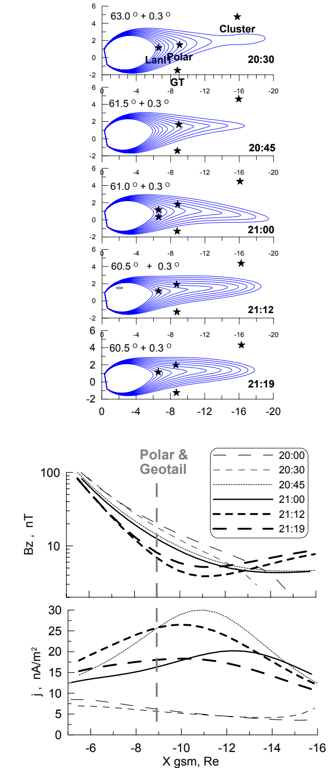
Fig. 11. Top: magnetic field line configurations (midnight XZ cross sections) during the substorm growth phase obtained from the adaptive modeling; CGLat of the innermost field line and latitudinal step between field lines are shown for each configuration. Bottom: time evolution of the radial current density profiles and B_Z profiles in the neutral sheet.
