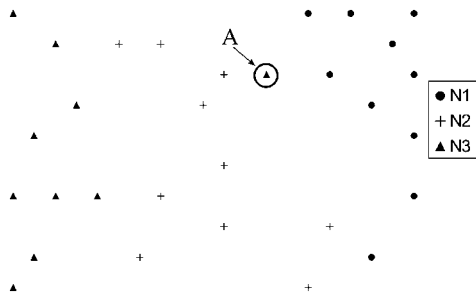
Fig. 8. Best-matching units in new map for each data set. Diagram is constructed from parameters sGL, nQT, and mQT, which were determined as most successful distinctive parameters from component planes of SOM. Only ash particle labeled 'A' is positioned in wrong field, due to its similarity in surface texture with this group. Note optimization as compared with that in Fig. 3.
