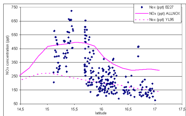
Fig. 7. \text{NO}_x concentrations in ppt from the UK BAe data between 450 and 650 m ASL, flight B227 (in blue), from the ALLNOX simulation (full purple line), and from the YL95 simulation (dotted purple line) at 500 m ASL
