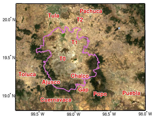
Fig. 1. Map of the MCMA and surrounding areas showing the T0, T1 & T2 supersites and surrounding cities (Puebla, Toluca, Cuernavaca, Pachuca and Tula). Terrain features shown are the Popocatepetl volcano, the Ajusco mountain and the gap in the southeast basin rim near Chalco. Political border of the MCMA as of 2003 in pink, background map is a MODIS true colour image from March 2006.
