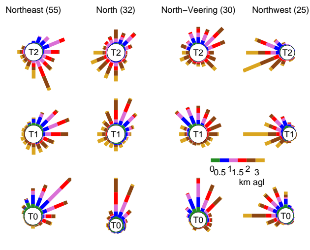
Fig. 8. Wind roses of the vertical wind profiles at T0, T1 and T2 for the Northerly flow clusters. Wind rose categories by height above ground level. Number of profiles in each cluster in parentheses.
