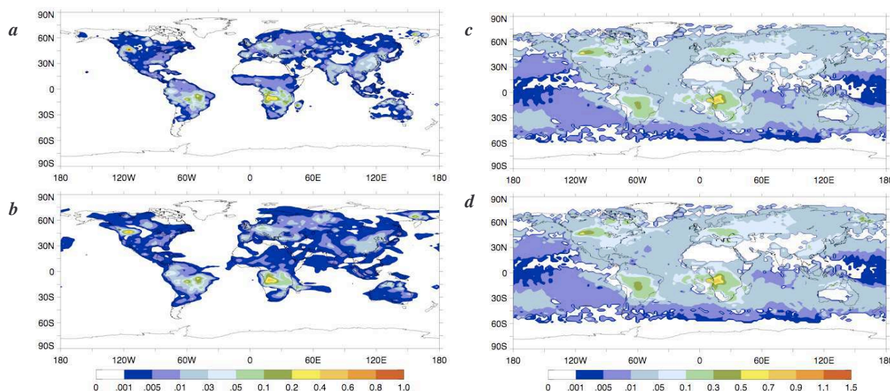
Fig. 12. Inversion test for retrieving daily emissions of a fine-mode BC component, using actual MODIS data sampling for August 18–30, 2000. Results are shown here for the two week average of retrieved daily emissions. (a) Two week average of assumed aerosol source distribution from GOCART model (emissions units: 10^7 kg/day). (b) Two week average of the retrieved aerosol source distribution for the same period. (c) Two week average of initial daily distributions of global aerosol optical depth. (d) Two week average of daily distributions of global aerosol optical depth simulated from retrieved sources.
