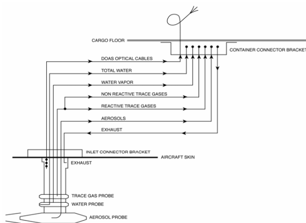
Fig. 5. Tubing connecting the inlet with the container connector bracket. The 3 optical fiber cables are continuous from the telescopes in the inlet to the spectrographs in the container.
