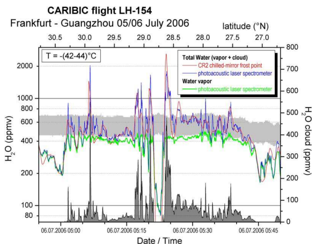
Fig. 8. The potential of both measuring gaseous water and total water using fast detector illustrated by the detection of cirrus clouds over China at \sim 11.4 \text{ km} pressure altitude. The grey band is the range between 100% saturation relative to ice and water. The photoacoustic signal (green) for water vapor reaches saturation versus ice at 05:02 UTC–05:20 UTC and 05:23 UTC–05:42 UTC. The photoacoustic signal for total water (blue, vapor plus ice crystals) exceeds the vapor signal during these two periods, although otherwise agreement is close (the difference of total and gaseous water signals is shown as a grey signal at the bottom). This indicates that 2 fields of cirrus clouds were intercepted. The photoacoustic measurements are fast ( <5 \text{ s} response time), while the chilled mirror hygrometer (red) shows “overshooting” (e.g. at 05:22 UTC) which is typical for this instrument type.
