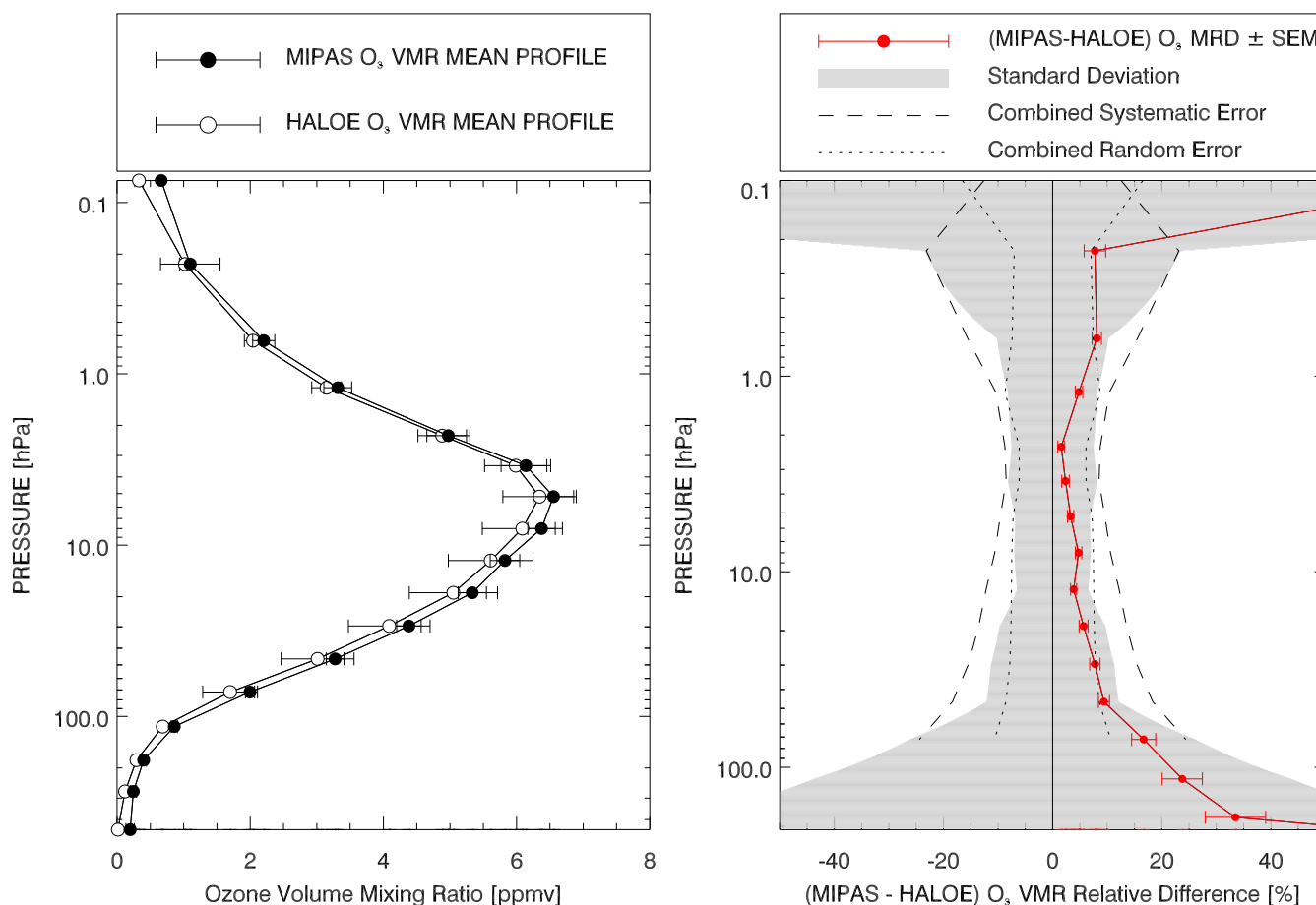
Fig. 27. Comparison between MIPAS and HALOE: statistics over all the collocated O 3 profiles.
