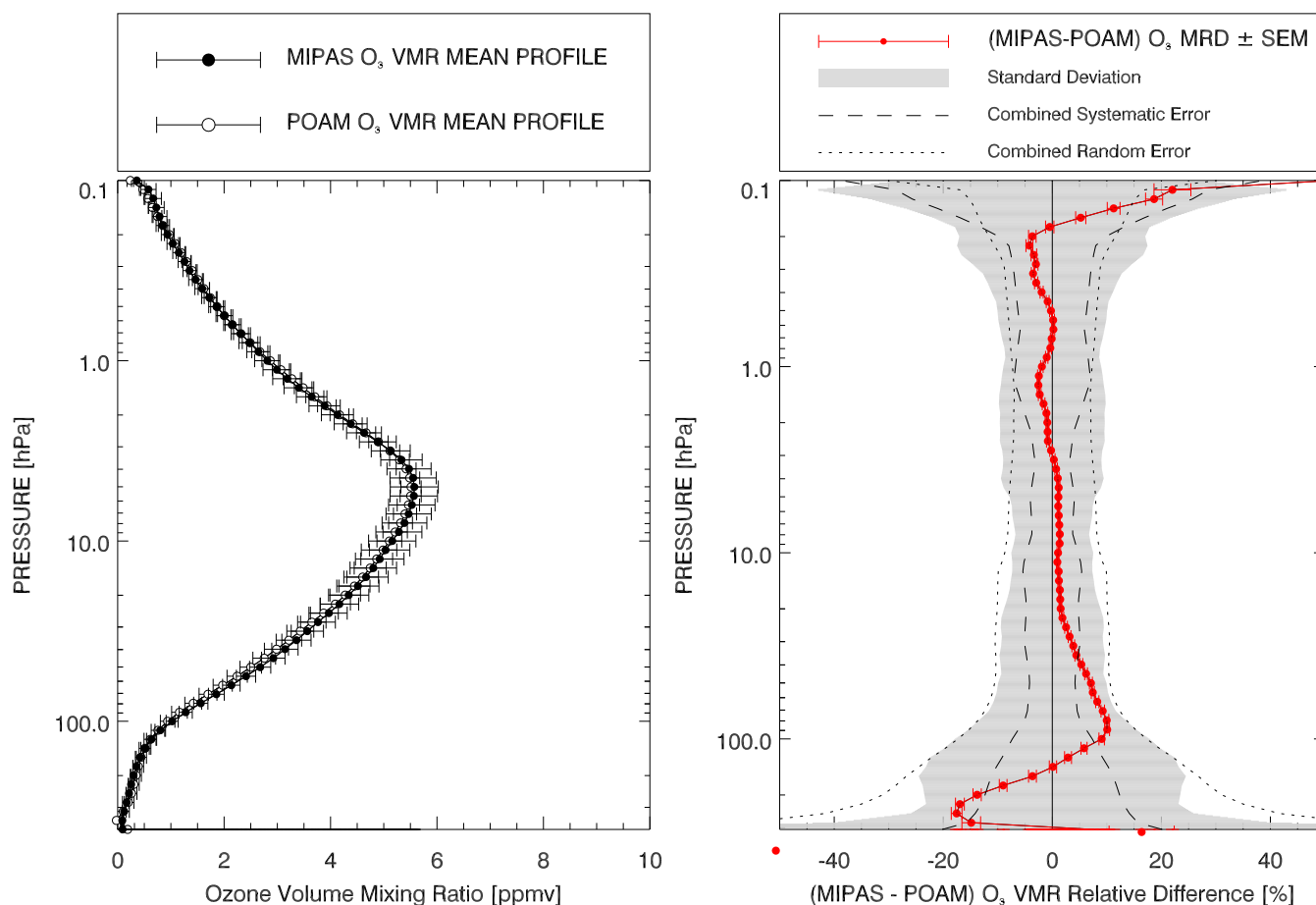
Fig. 22. Comparison between MIPAS and POAM III: statistics over all the collocated \text{O}_3 profiles. Global mean profiles of \text{O}_3 VMR measured by MIPAS and by POAM III, with error bars indicating the corresponding total uncertainties (left panel). Mean relative difference between MIPAS and POAM III ozone data and combined error budget (right panel).
