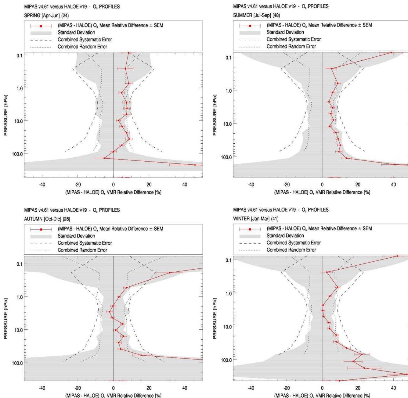
Fig. 29. Comparison between MIPAS and HALOE \text{O}_3 profiles: seasonal averages.
