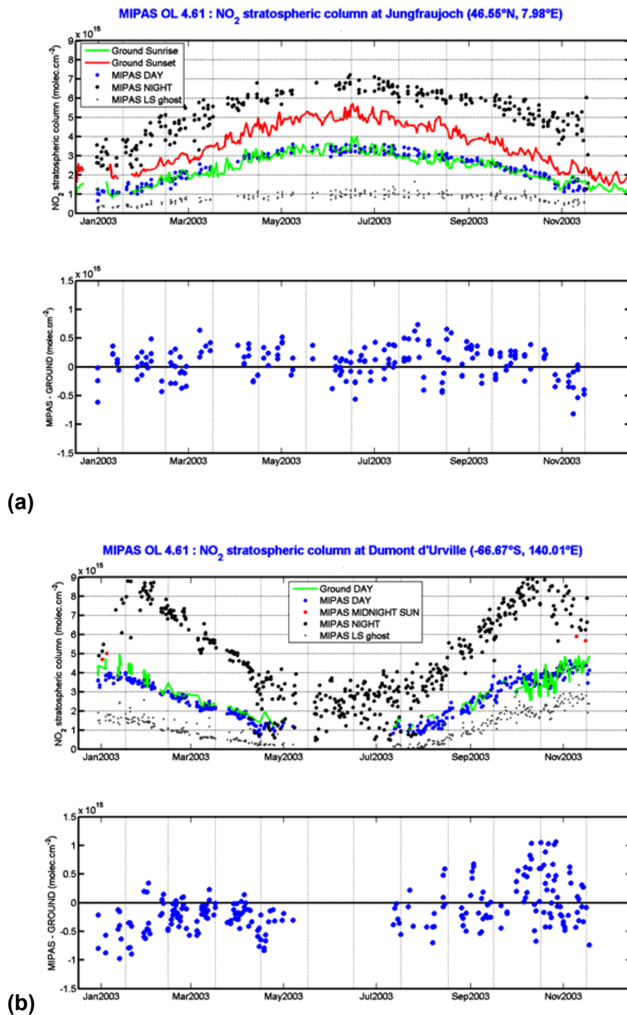
Fig. 18. Seasonal variation in 2003 of the absolute difference between MIPAS version 4.61 and ground-based DOAS/UV-visible NO 2 column data at the NDACC stations Jungfrauoch (Swiss Alps) and Dumont d'Urville (French Antarctica). Ground-based morning (sunrise), afternoon (sunset) and UV-visible column (photochemically corrected with respect to MIPAS day) measurements are shown together with MIPAS day, night, and midnight sun observations and the lower stratospheric "ghost" column (panel a, top, and b, top). Differences are shown between MIPAS (day) and ground-based (sunrise) observations (panel a, bottom) and between MIPAS (day) and ground-based UV-visible column (panel b, bottom).
