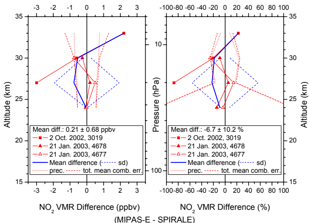
Fig. 5. Differences of all comparisons between SPIRALE and MIPAS-E. An ascent profile of SPIRALE from 2 October 2002 is compared to a MIPAS-E limb scan performed during orbit 3019. The SPIRALE profile from 21 January 2003 has been compared to MIPAS-E observations carried out during orbits 4677 and 4678.
