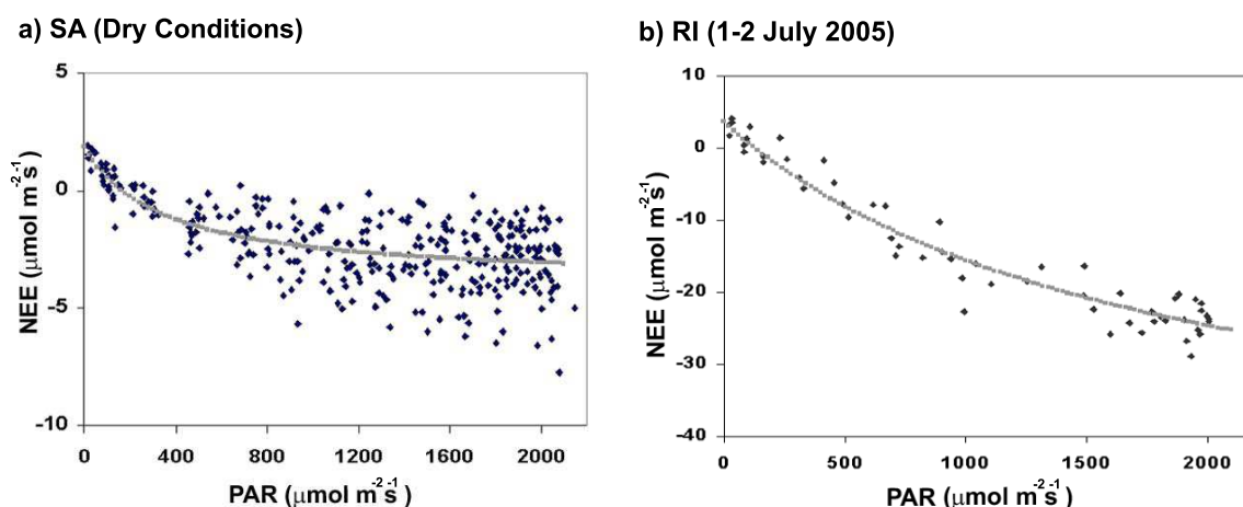
Fig. 2. Observed vegetation atmospheric CO 2 flux (NEE in \mu\text{mol m}^{-2} \text{s}^{-1} ) as a function of solar radiation in the PAR domain ( \mu\text{mol m}^{-2} \text{s}^{-1} ): (a) El Saler (SA in Fig. 1) during the days selected for driest conditions between June and August 2001, (b) the Rice tower (RI in Fig. 1) during 1–2 July.
