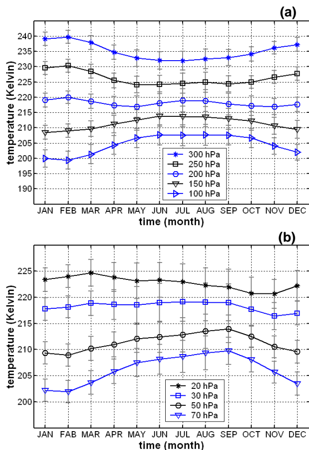
Fig. 2. Time evolution of monthly averaged temperatures per height: (a) in the upper troposphere and (b) in the lower stratosphere over Durban (see legends).
