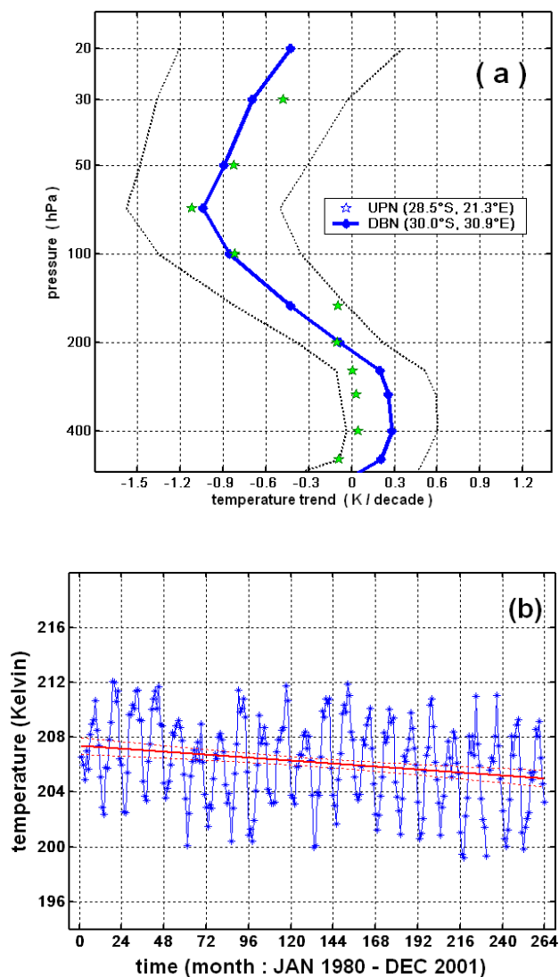
Fig. 4. (a) Linear temperature trend (in Kelvin per decade) height profile framed with the 95% confidence profiles, derived from Durban: DBN (30.0° S, 30.9° E) morning data. Uppington (UPN: 28.5° S, 21.3° E) trends retrieved from during January 1980–March 1999 period are shown with star symbols. (b) Time evolution of the monthly averaged temperature values in the lower stratosphere (at 70 hPa), over Durban. The superimposed red line indicates the obtained linear trend, i.e., -1.09 \pm 0.41 K per decade.
