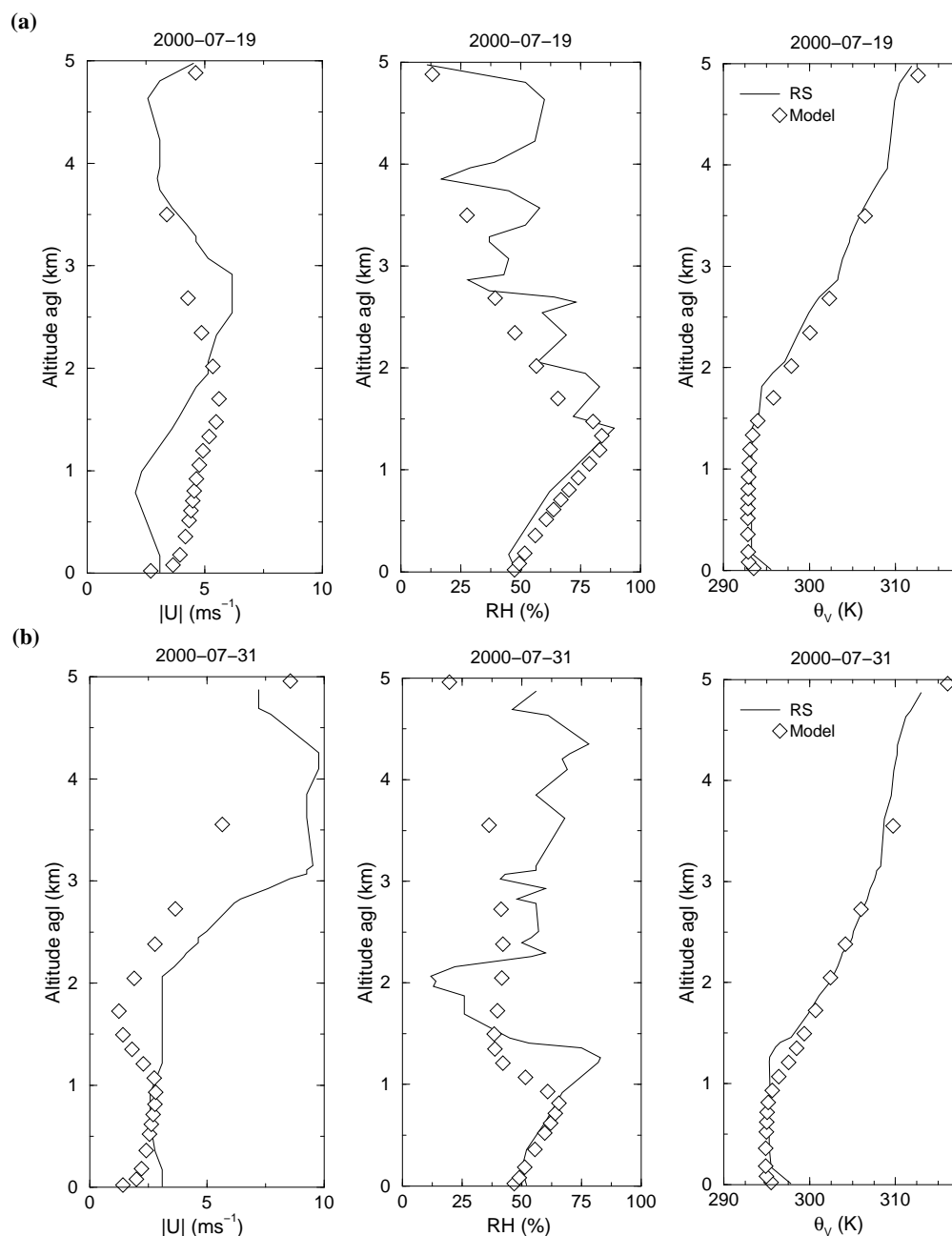
Fig. 5. Vertical profiles of wind speed ( U ), relative humidity ( RH ) and potential temperature ( \Theta_V ) observed by Trappes ( 48.78^\circ \text{ N} , 2^\circ \text{ E} ) radiosoundings (solid line) and simulated by the model (diamonds) on 19 (a) and 31 (b) July 2000.
